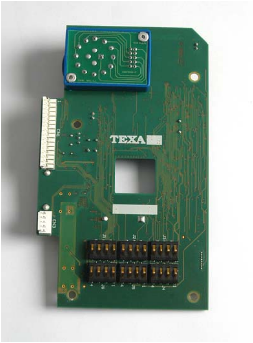
Main board bottom
