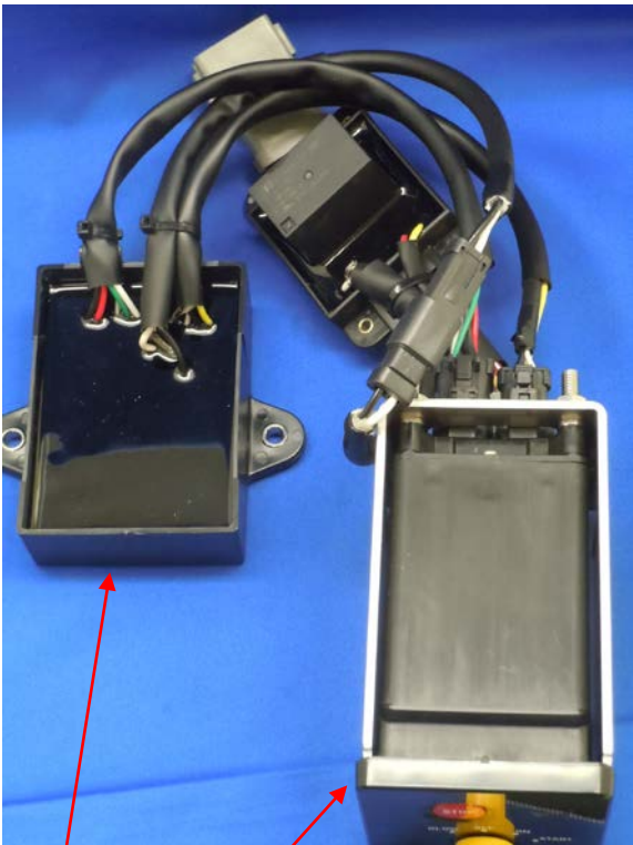
CZ175 Panel Switch (incl. Antenna)
