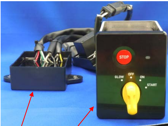
CZ175 Panel Switch (incl. Antenna)
