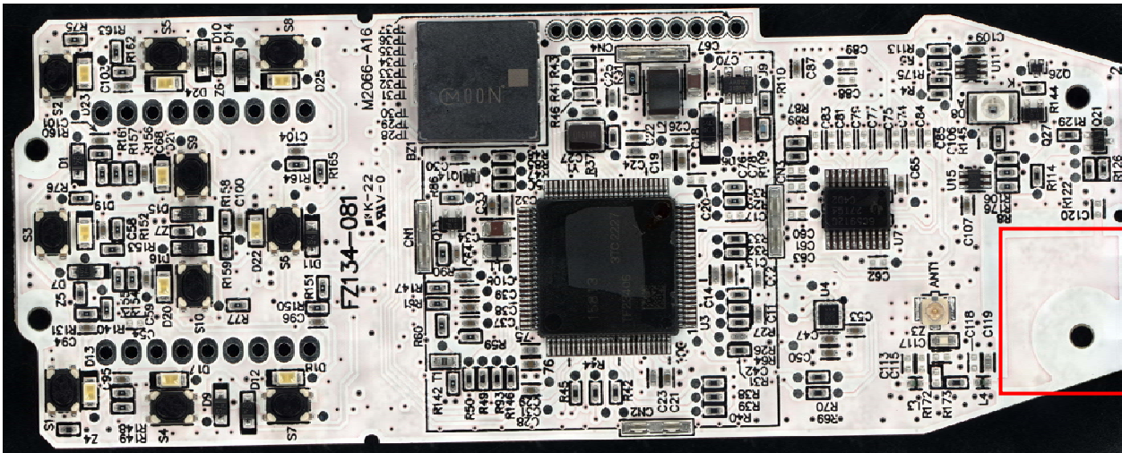
Bluetooth Pattern Antenna
