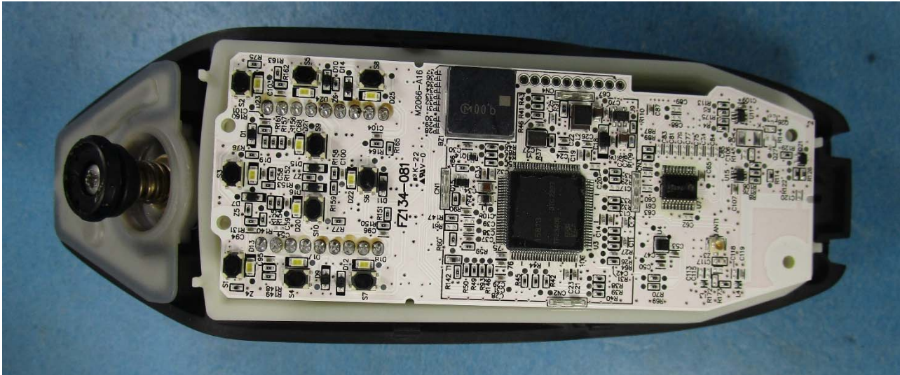
Bluetooth Pattern Antenna
