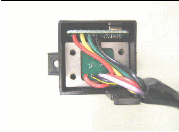
KZ42 Immobilizer Internal photograph(PWB)
