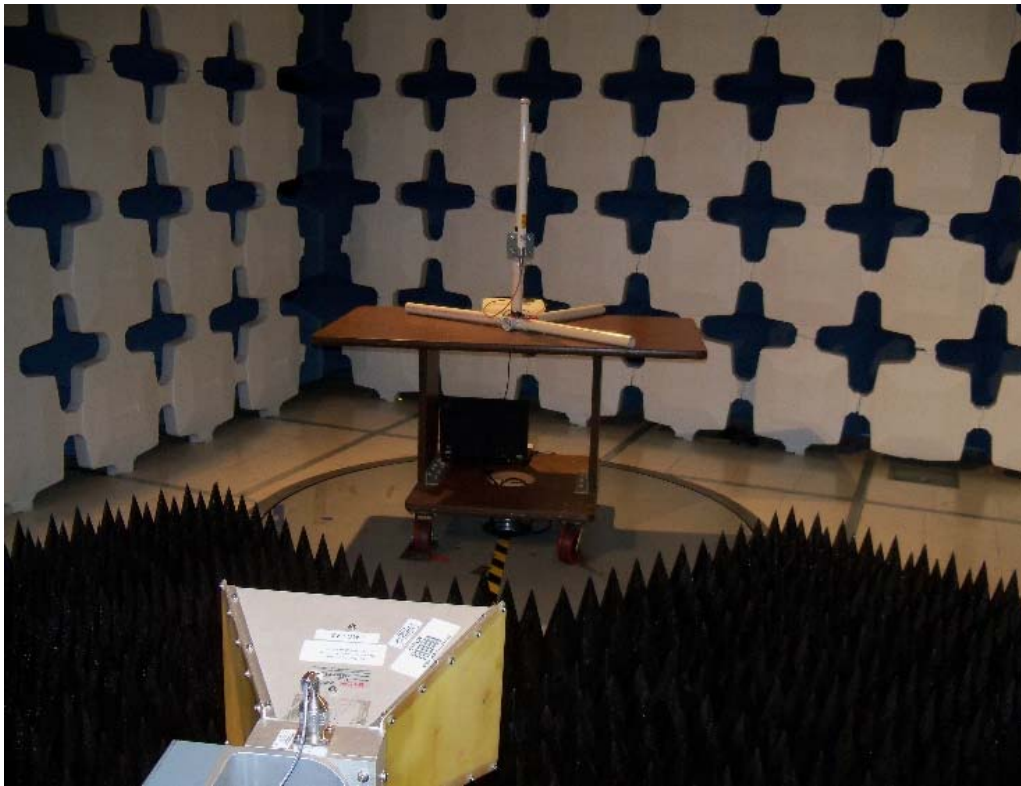
Test Setup Photos Microchip
