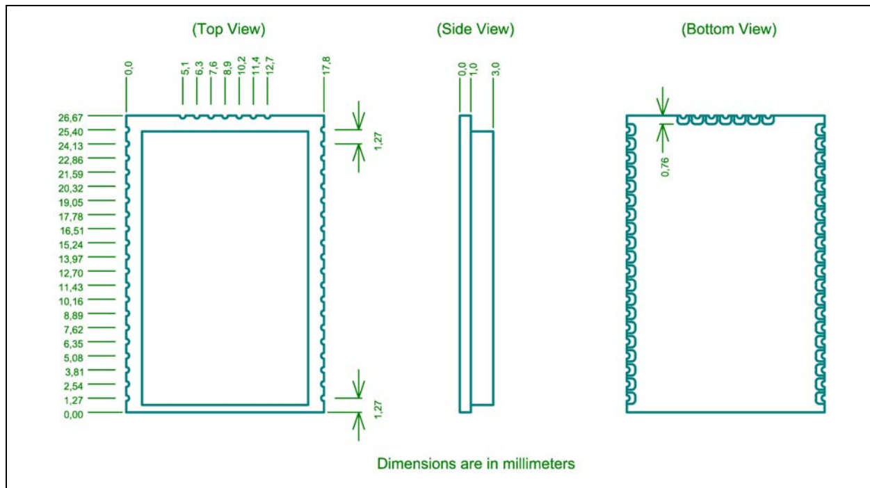
FIGURE 4-1: RN2903 PHYSICAL DIMENSIONS
