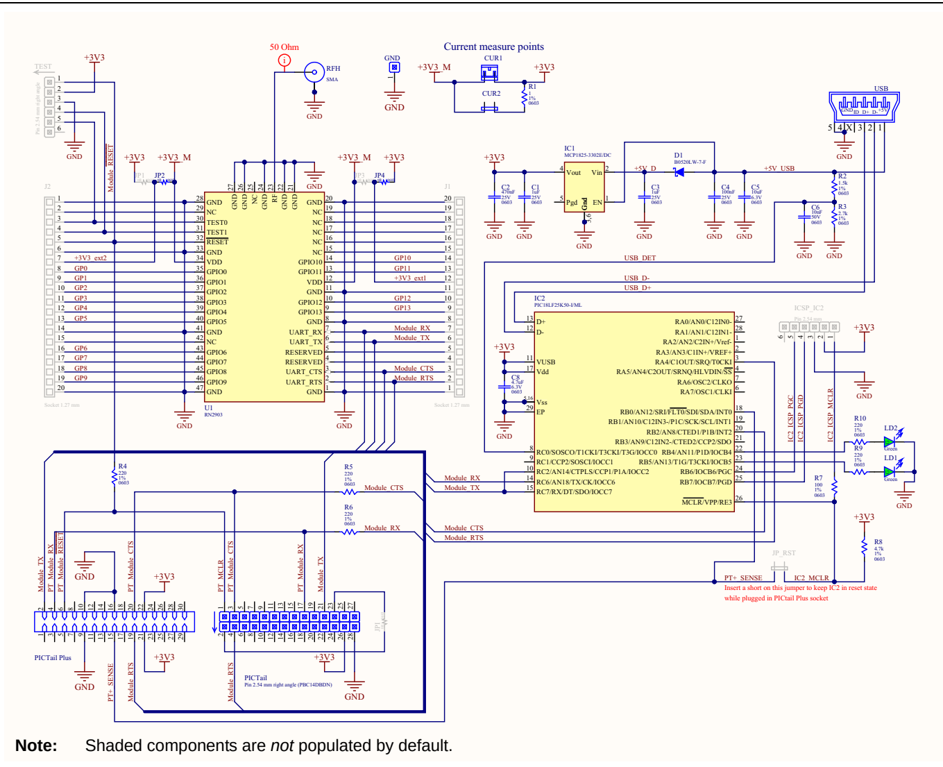
FIGURE 5-2: PICTAIL™/PICTAIL PLUS DAUGHTER BOARD SCHEMATIC
