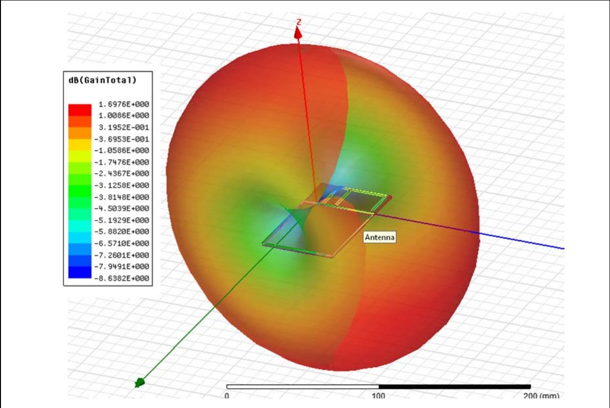
FIGURE 5-5: SIMULATED THREE DIMENSIONAL RADIATION PATTERN
