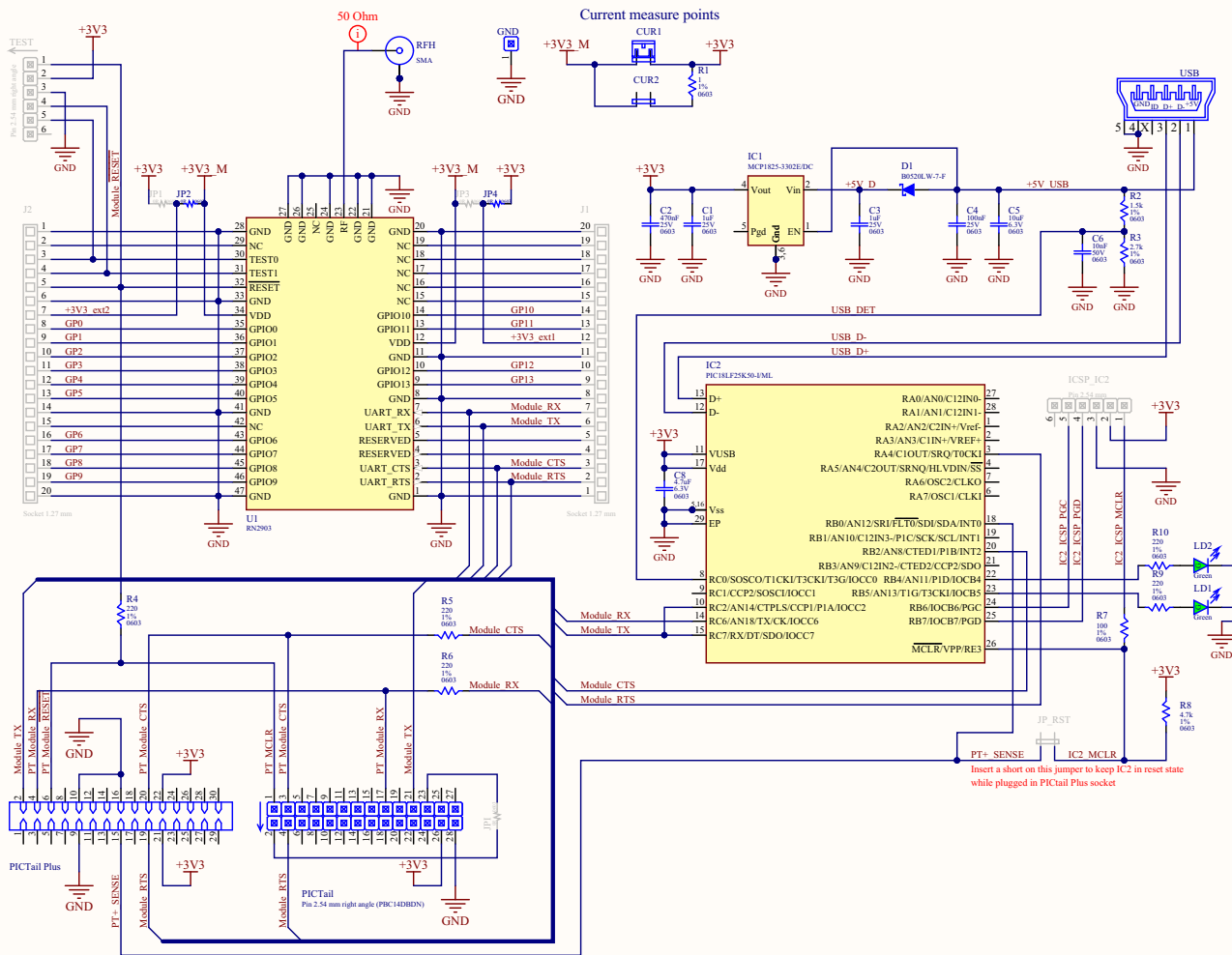
FIGURE 5-6: PICTAIL™/PICTAIL PLUS DAUGHTER BOARD SCHEMATIC
