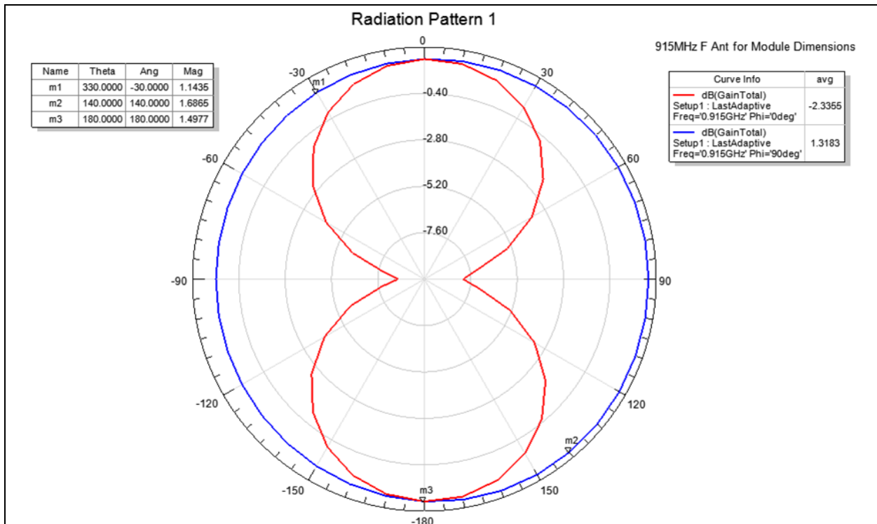
FIGURE 5-4: SIMULATED TWO-DIMENSIONAL RADIATION PATTERN
