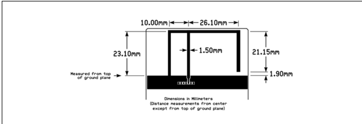
FIGURE 5-3: PCB TRACE ANTENNA MEASUREMENTS
