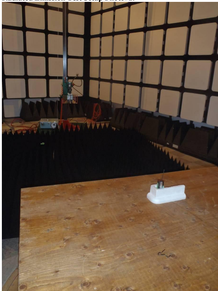
Radiated Emission Test Setup Photo#2:
