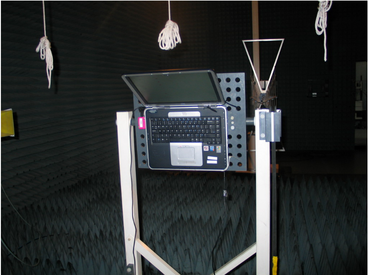
Photo 5: Setup for radiated tests
