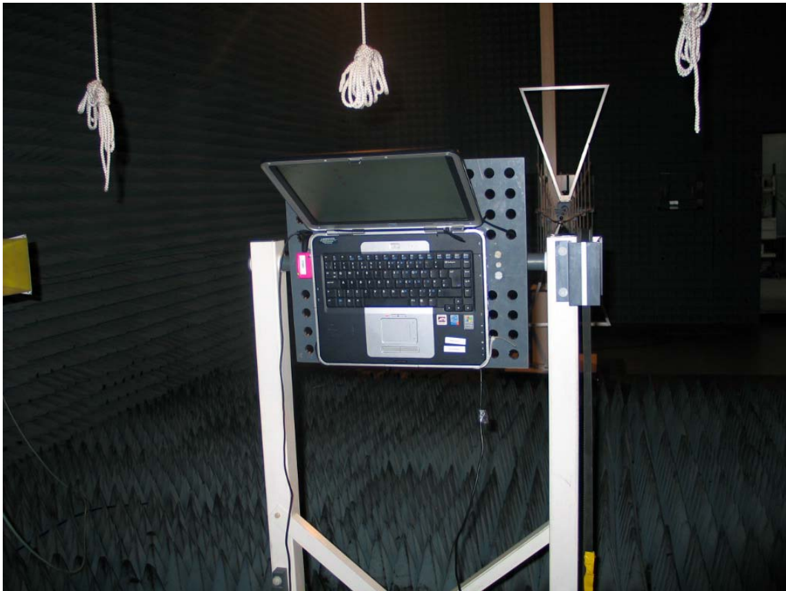
Photo 5: Setup for radiated tests
