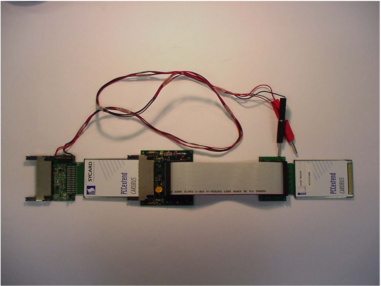
Photo 4: Cradle, used for conducted tests
