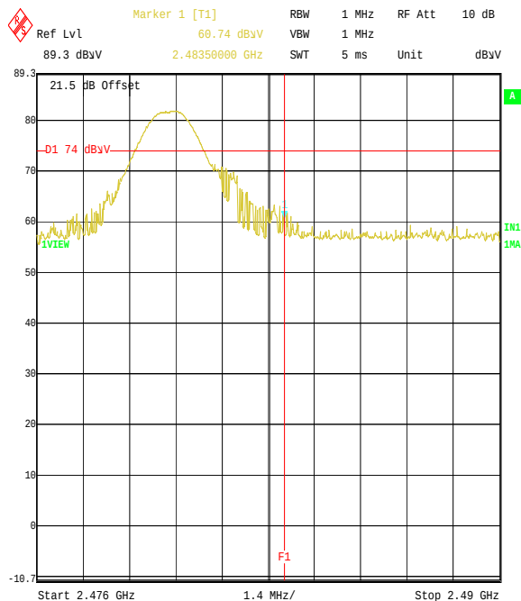
Title: Crane Electronics FCC Part 15.247 Electronic Torque Wrench Comment A: Radiated Band Edge on Static Mode Top Channel Date: 13.MAY.2005 12:27:43
