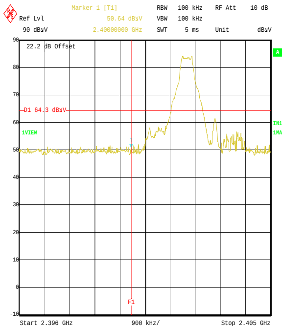
Title: Crane Electronics FCC Part 15.247 Electronic Torque Wrench Comment A: Radiated Band Edge on Static Mode Bottom Channel Date: 13.MAY.2005 12:23:59
