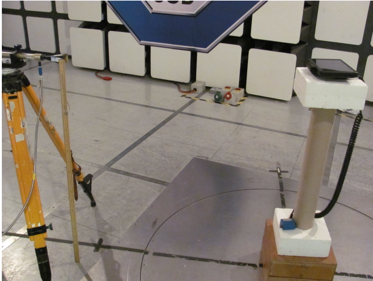
Radiated Emissions 18-25GHz
