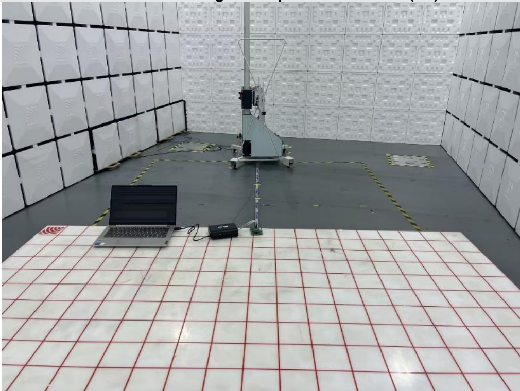
Radiated Band edge and Spurious Emission (BT)
