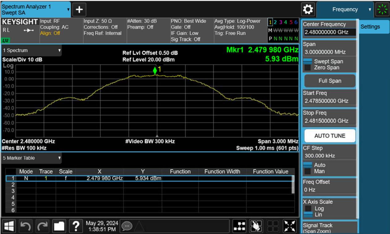
Figure 69: Conducted Spurious Emission & Authorized-band band-edge, 2480MHz, BLE-1Mbps Carrier Level
