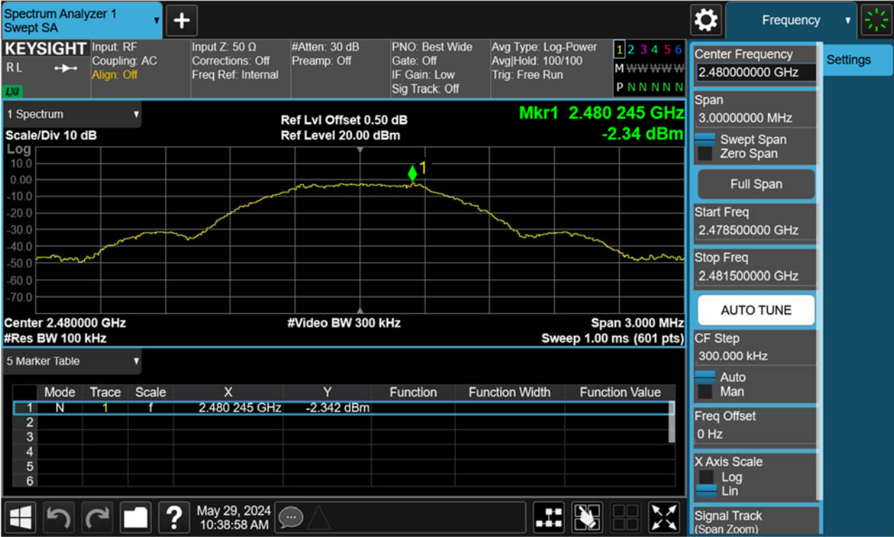
Figure 63: Conducted Spurious Emission & Authorized-band band-edge, 2480MHz, BLE-1Mbps Carrier Level
