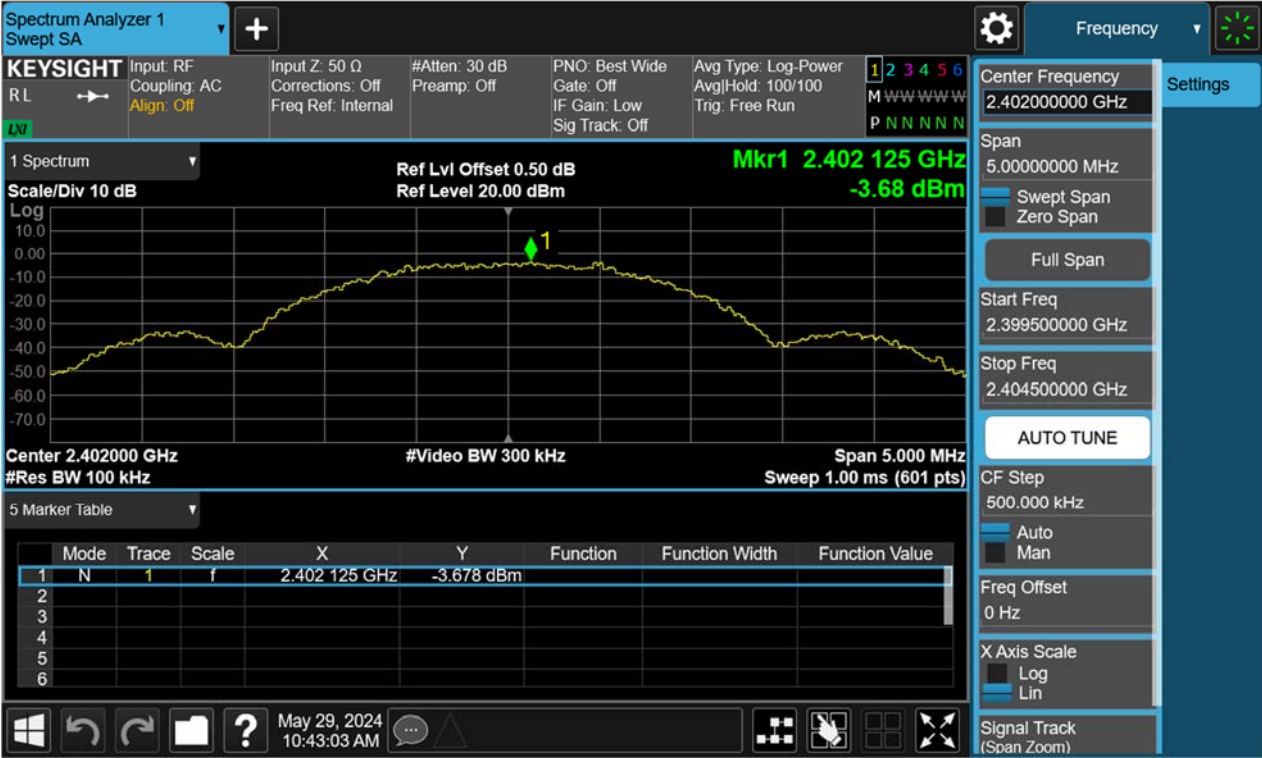
Figure 64: Conducted Spurious Emission & Authorized-band band-edge, 2402MHz, BLE-2Mbps Carrier Level
