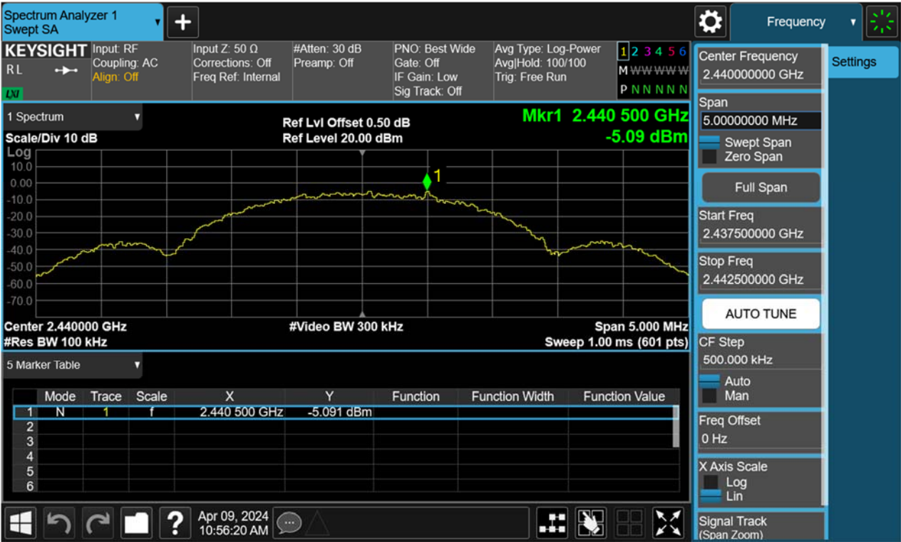
Figure 59: Conducted Spurious Emission & Authorized-band band-edge, 2440MHz, BLE-2Mbps Carrier Level
