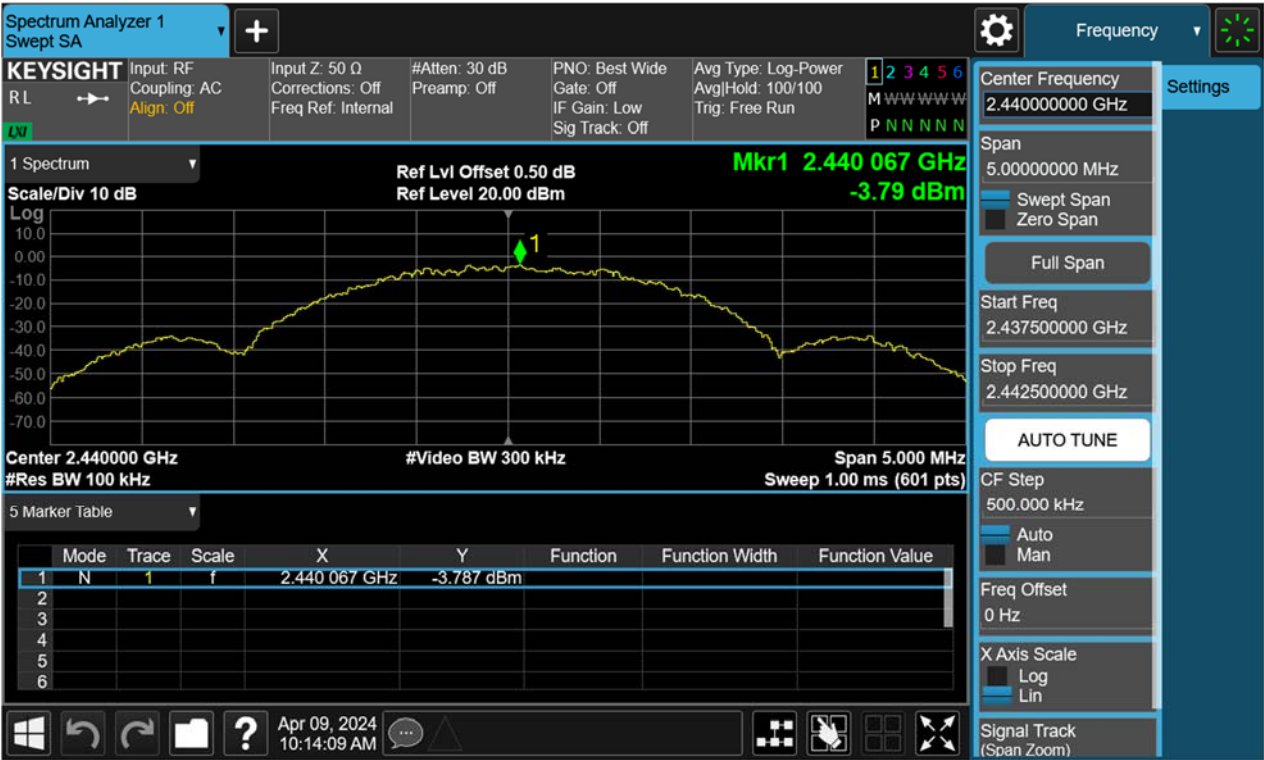
Figure 65: Conducted Spurious Emission & Authorized-band band-edge, 2440MHz, BLE-2Mbps Carrier Level
