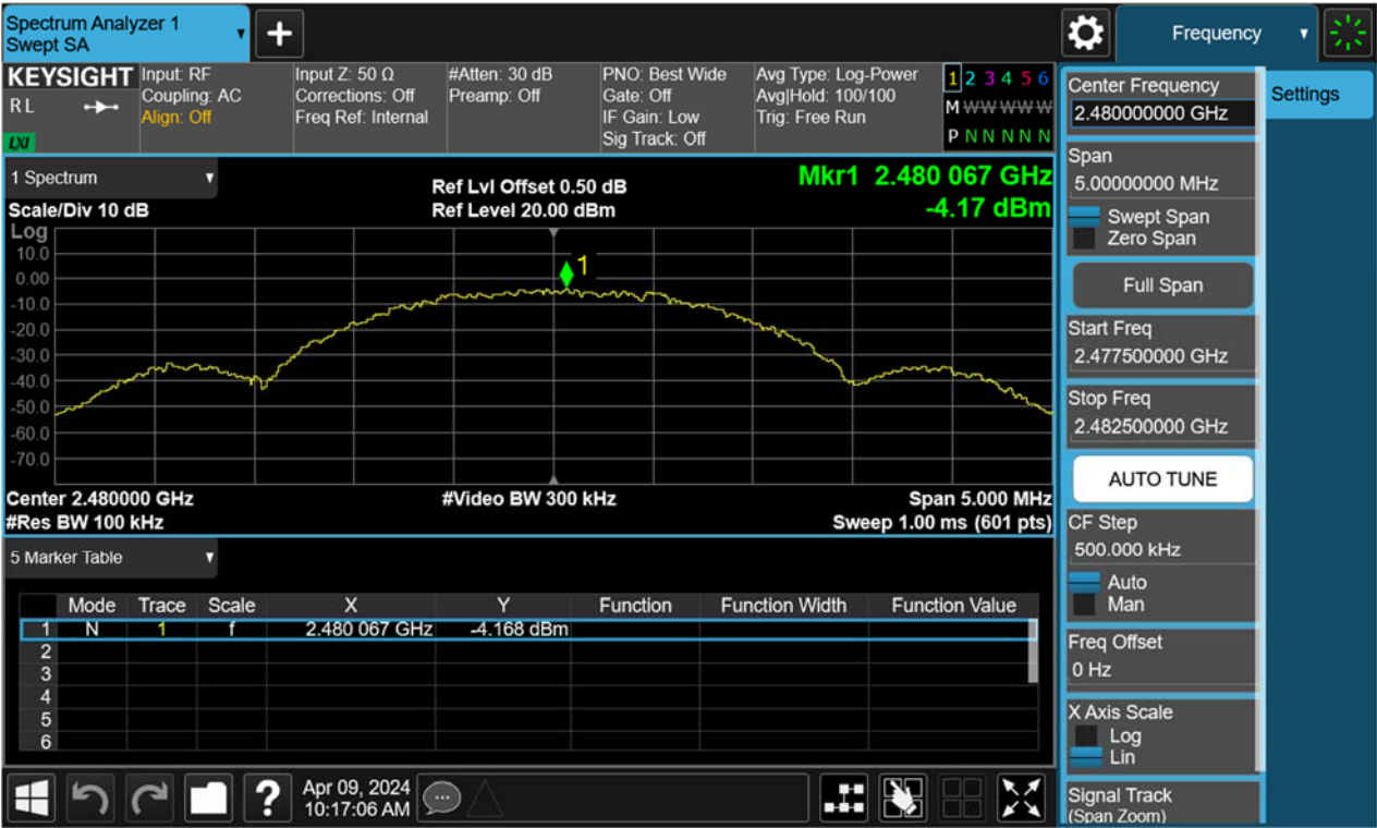
Figure 66: Conducted Spurious Emission & Authorized-band band-edge, 2480MHz, BLE-2Mbps Carrier Level
