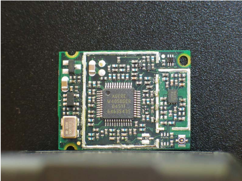
Module PCB top without shielding
