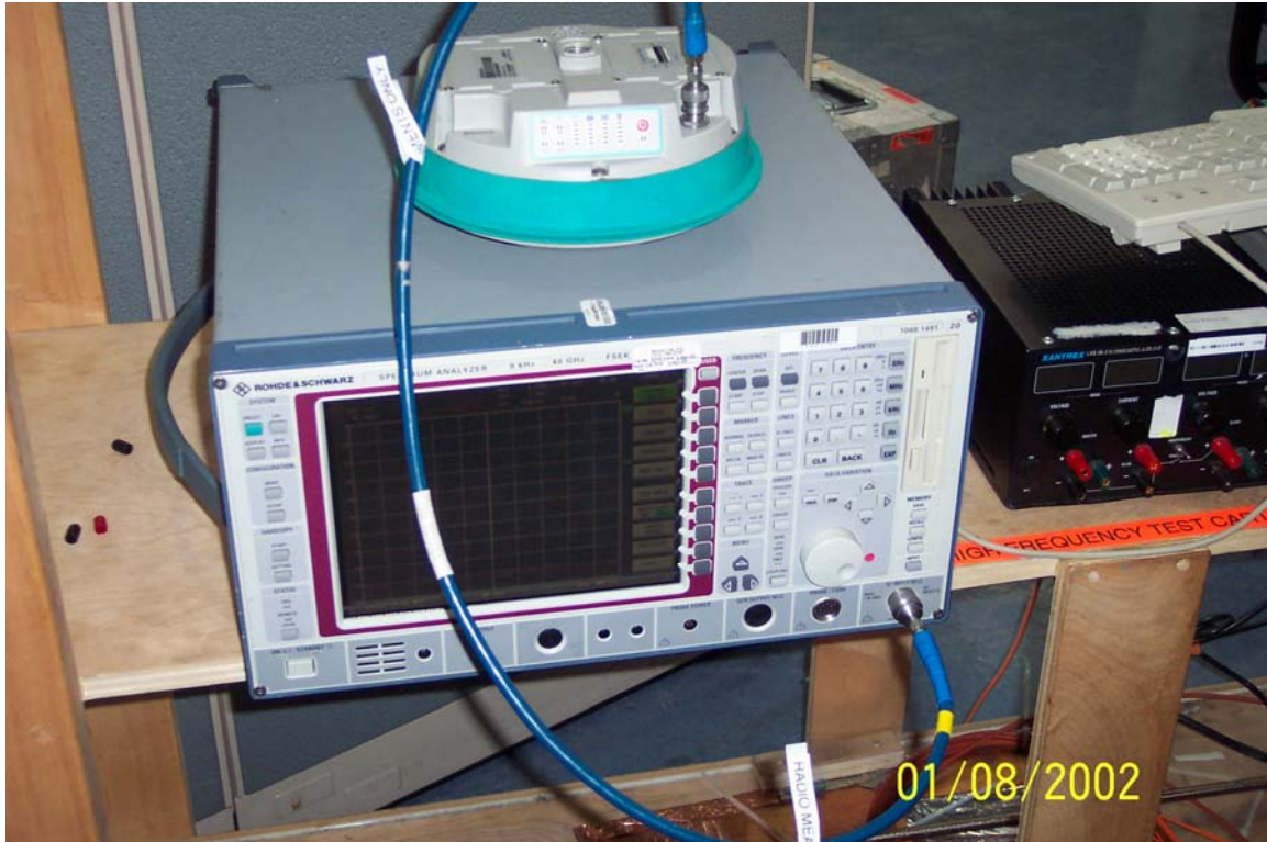
Figure 3 Conducted RF Setup
