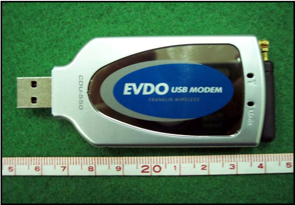
The Front View without Case
