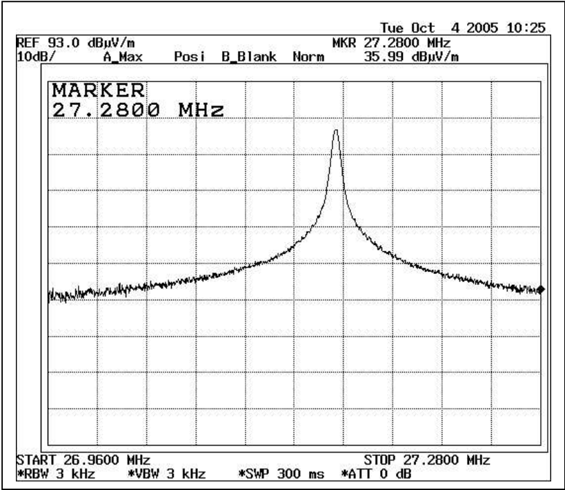
Bandwidth Plot
