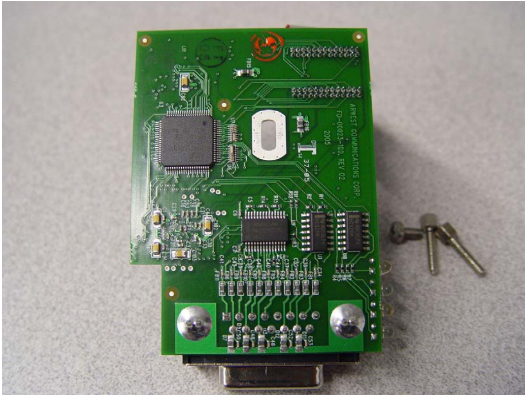
Daughter pcb underside
