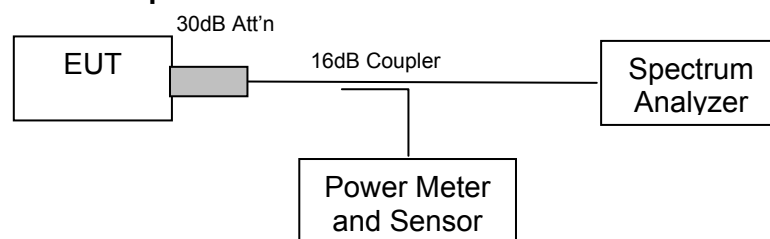
Test set up for Occupied Bandwidth and Emission Mask measurement
