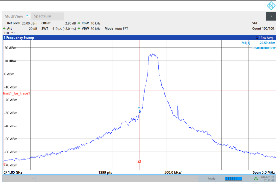
Band2-1.4MHz-QPSK-18607-1RB#0
