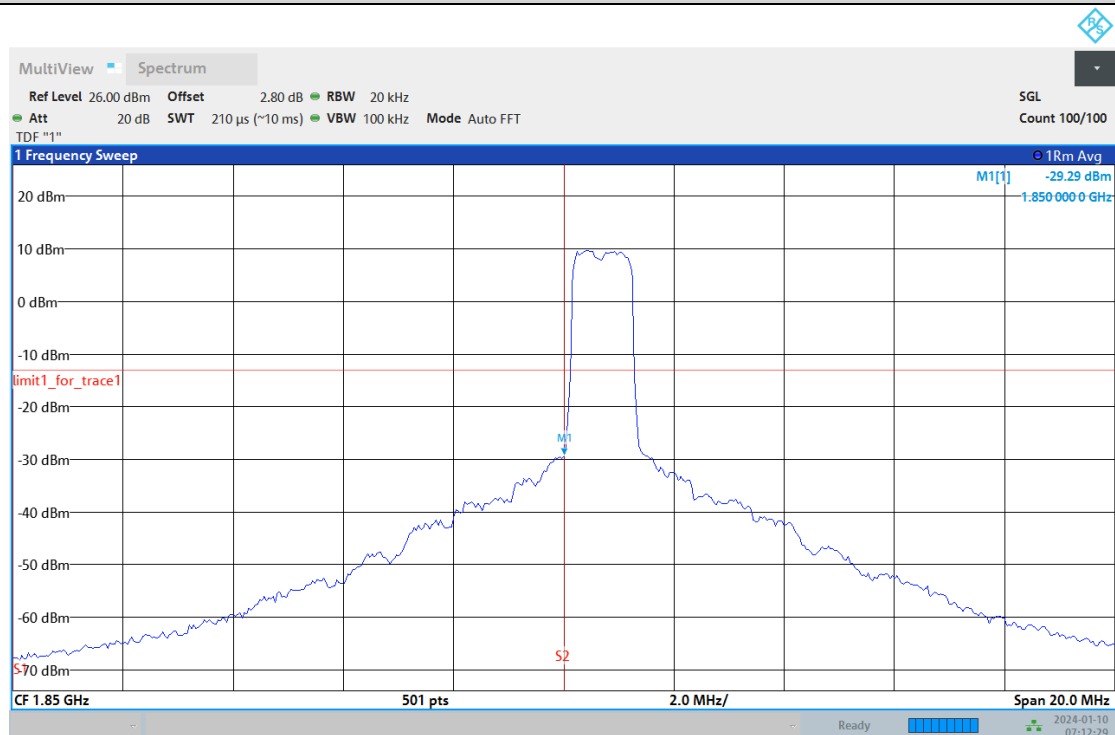
Band2-1.4MHz-QPSK-18607-6RB#0
