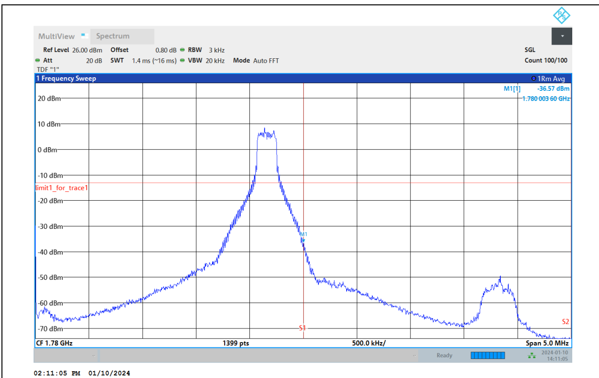
Band66-5MHz-QPSK-132647-25RB#0
