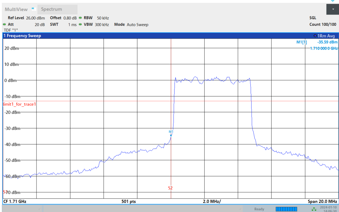
Band66-5MHz-QPSK-132647-1RB#24
