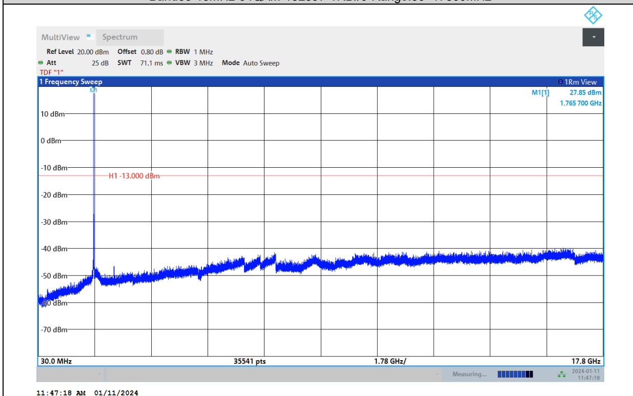
Band66-20MHz-QPSK-132072-1RB#0-Range:30~17800MHz
