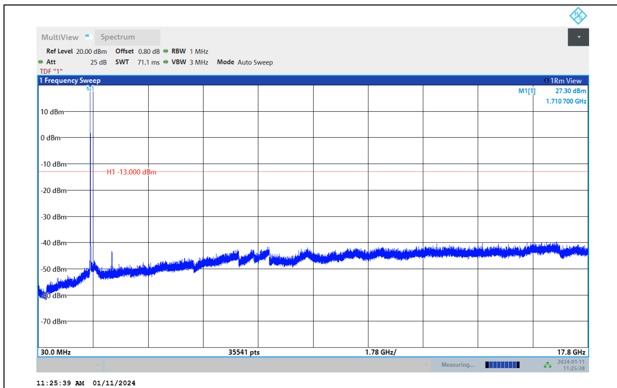
Band66-15MHz-QPSK-132322-1RB#0-Range:30~17800MHz
