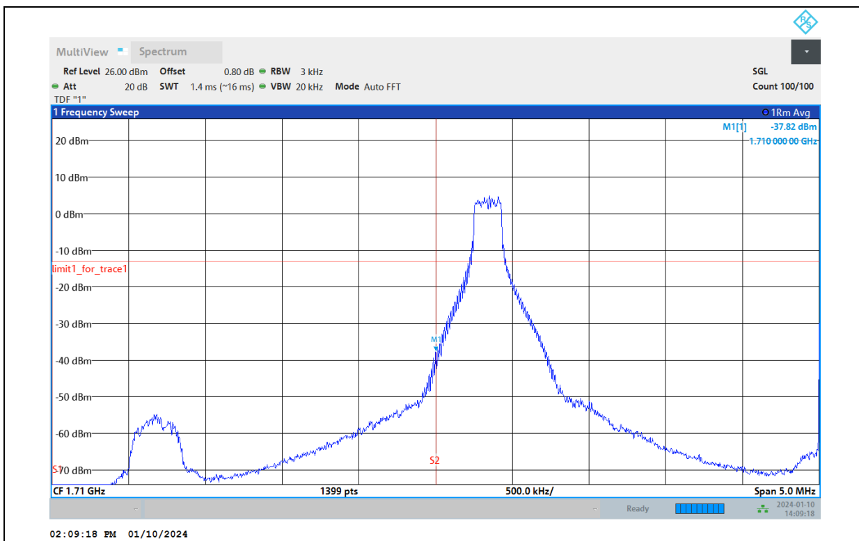
Band66-5MHz-64QAM-131997-25RB#0
