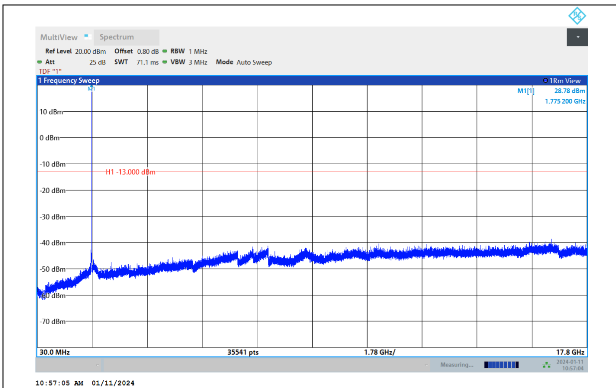
Band66-10MHz-QPSK-132022-1RB#0-Range:30~17800MHz
