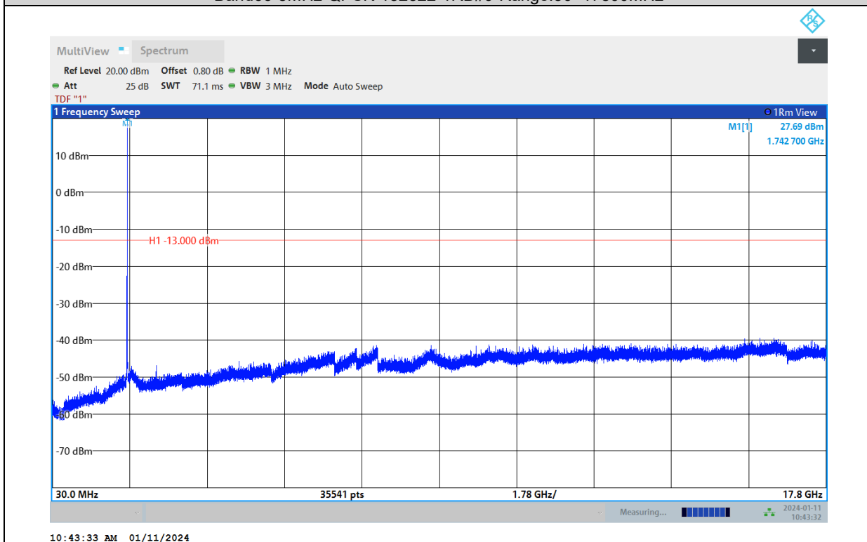
Band66-5MHz-QPSK-132647-1RB#0-Range:30~17800MHz
