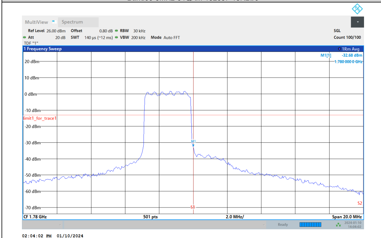
Band66-5MHz-QPSK-131997-1RB#0
