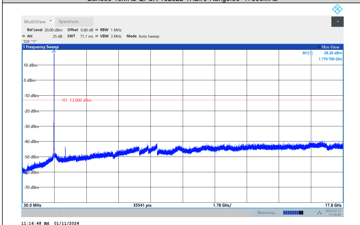
Band66-10MHz-16QAM-132622-1RB#0-Range:30~17800MHz
