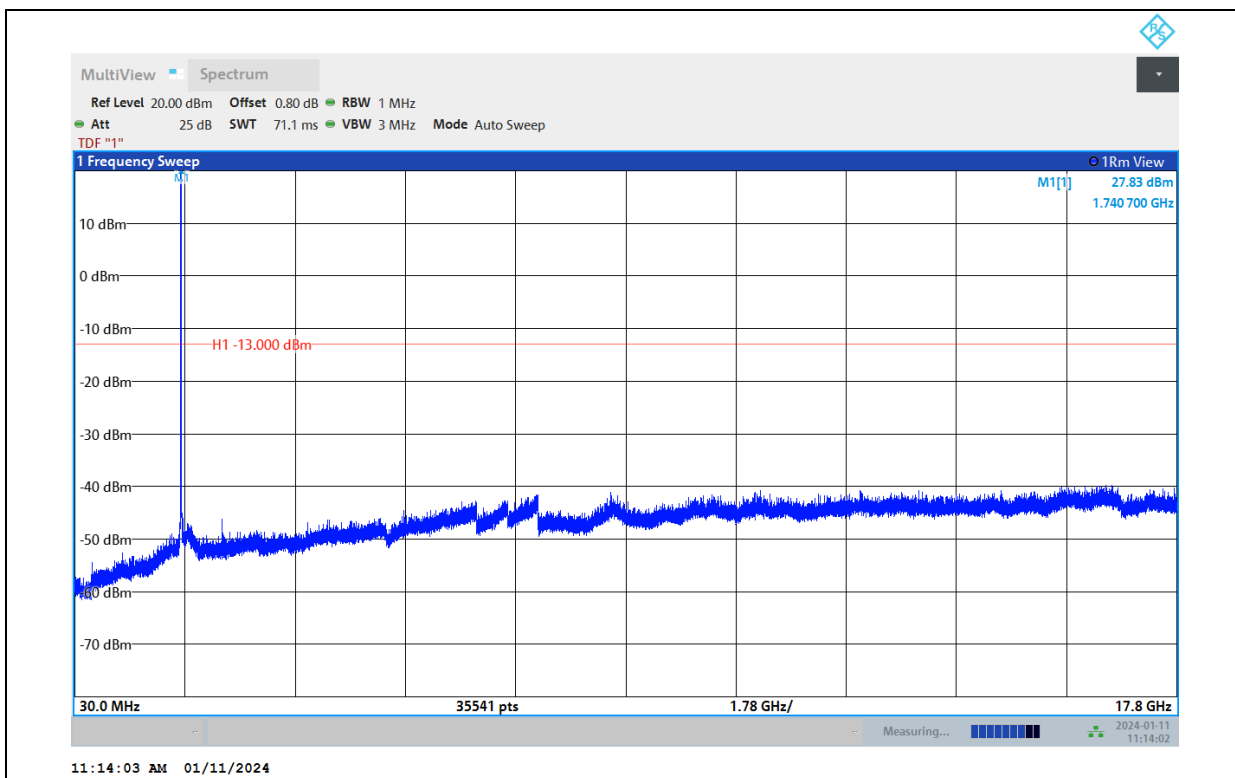
Band66-10MHz-64QAM-132622-1RB#0-Range:30~17800MHz
