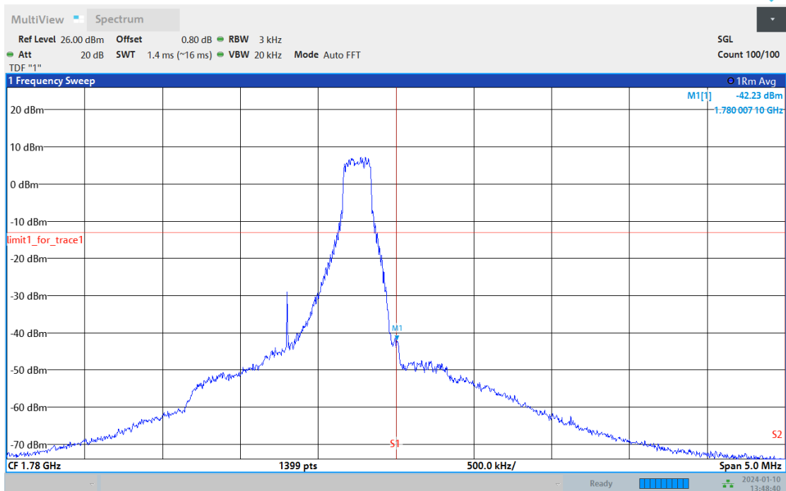
Band66-1.4MHz-QPSK-132665-6RB#0
