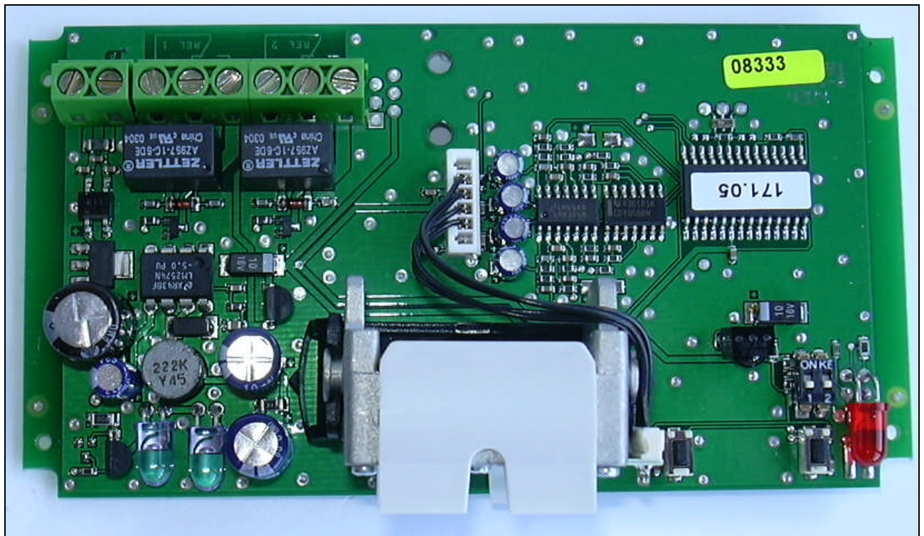
Photo 2: Top View
