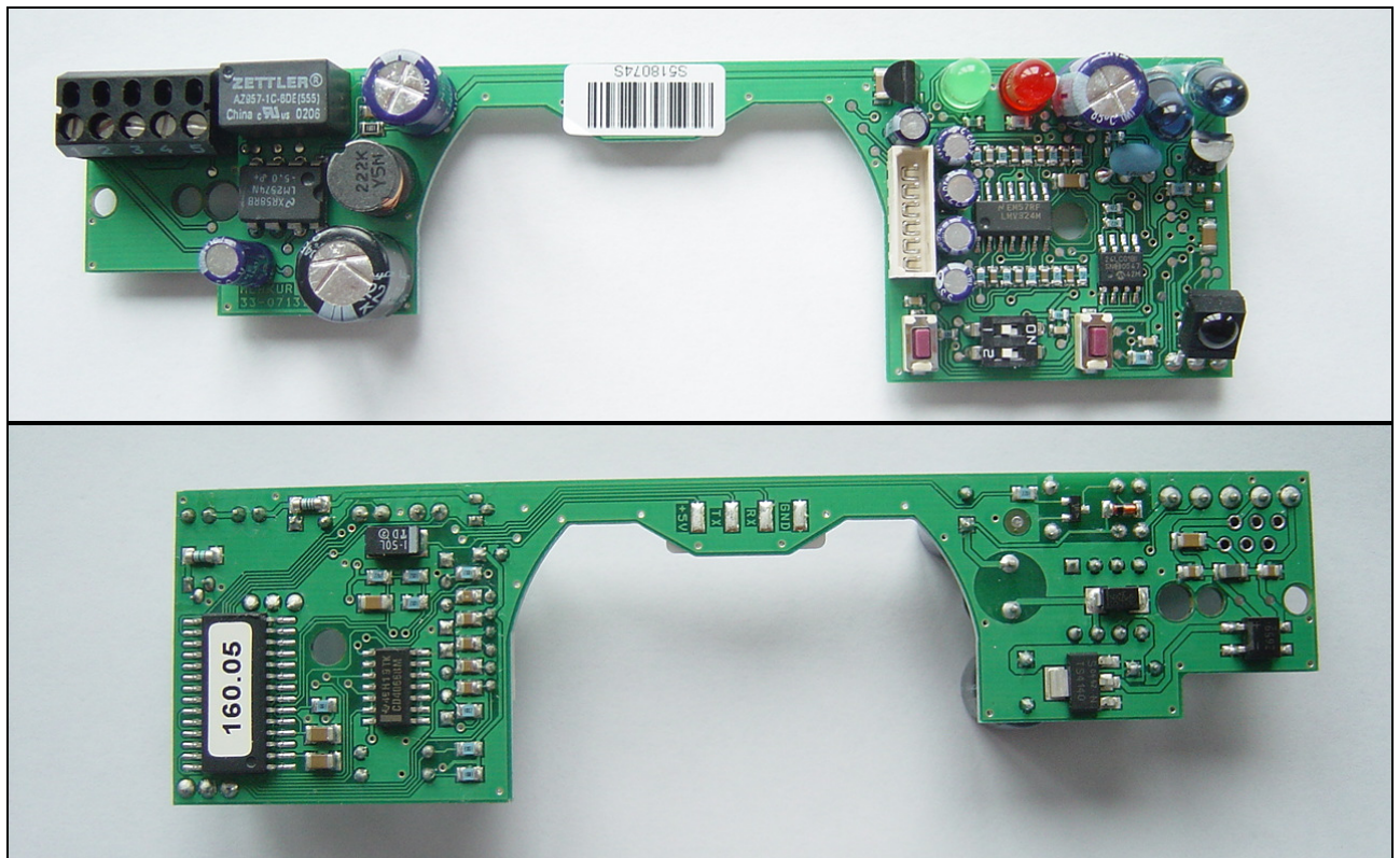
Photo 1: Bottom and Top View
