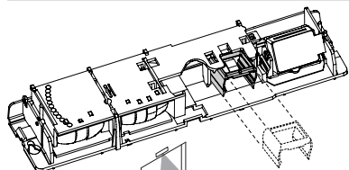
Clip in parking position
