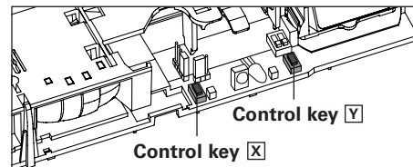
Control keys
