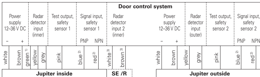
Connection principle
