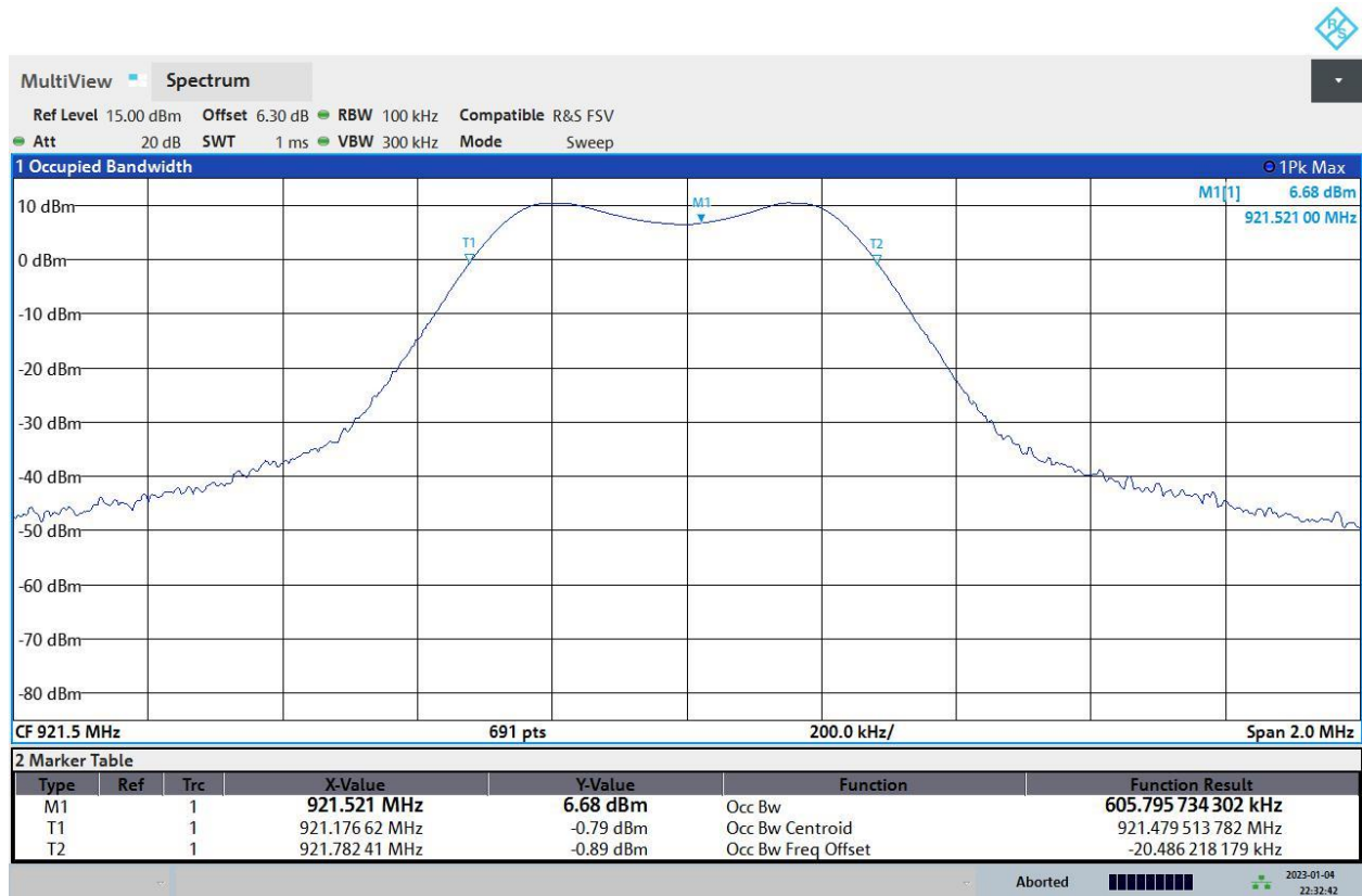
Figure 2: D001_99%OBW
