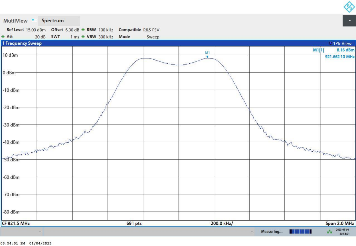
Figure 5: D005_01_sweep_ref
