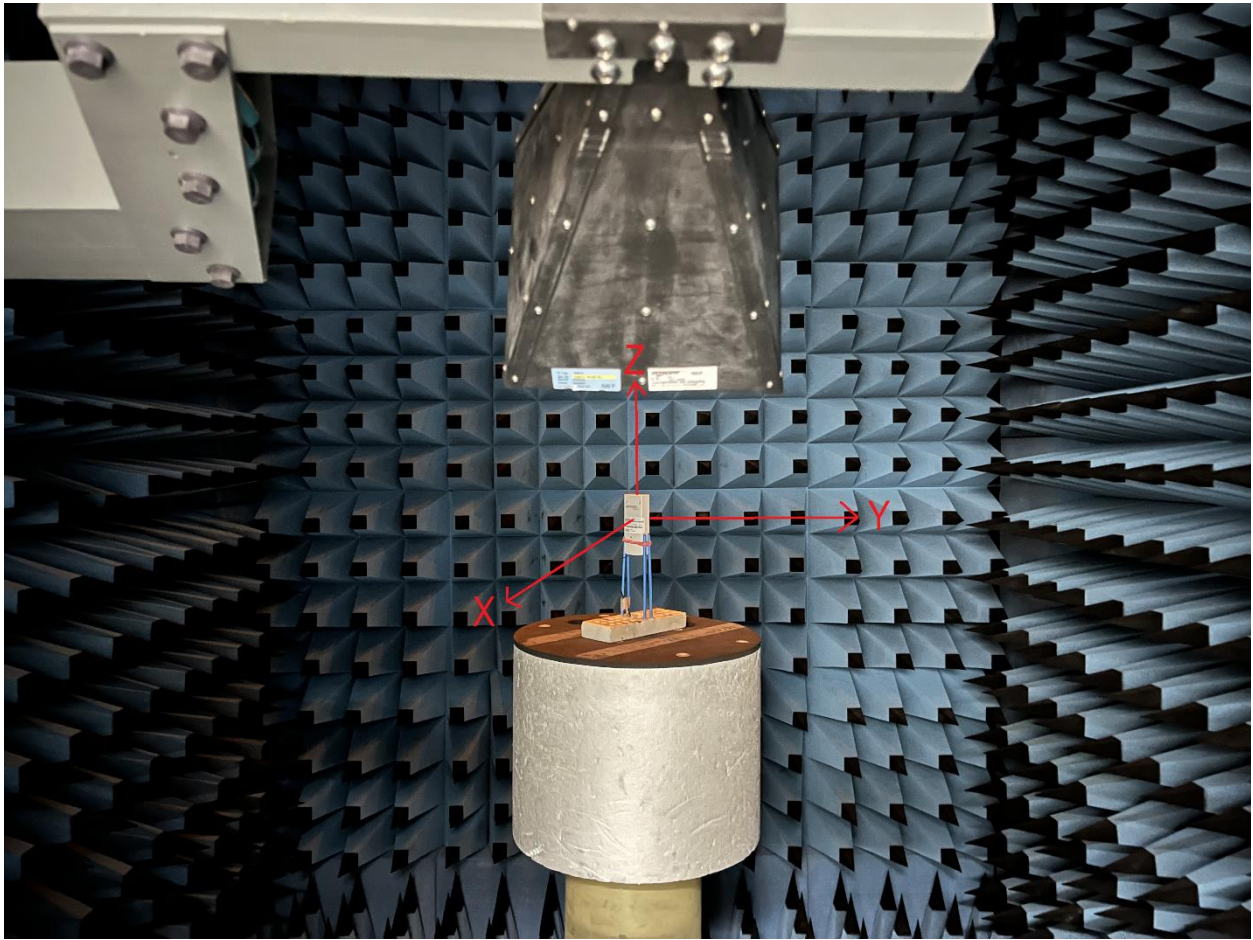
Photograph 3: EUT test setup 3D OTA test
