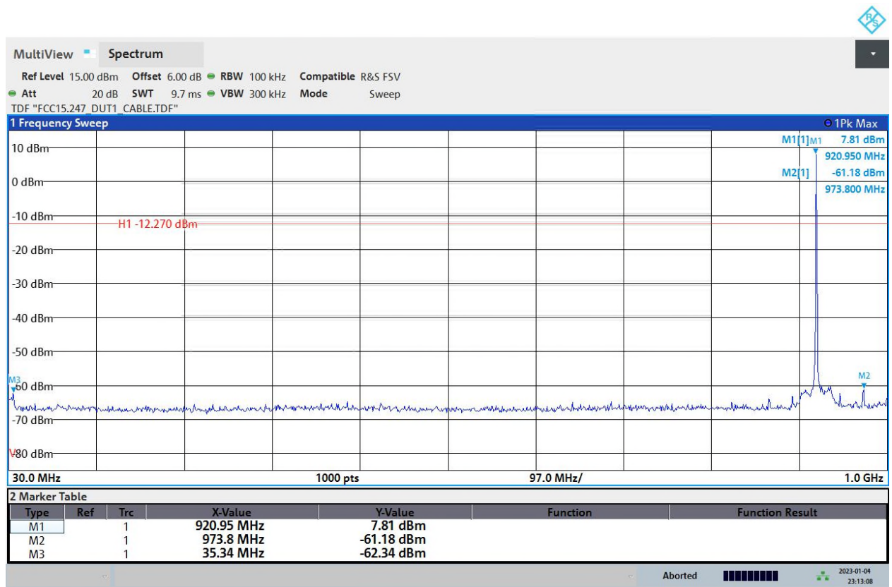
Figure 7: D005_03_sweep_2
