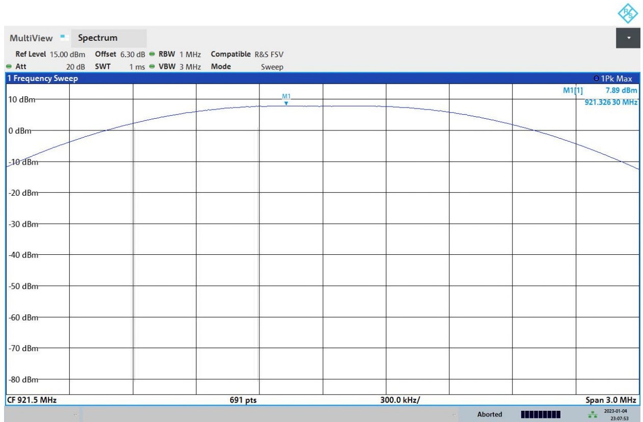
Figure 3: D003_PK-PWR
