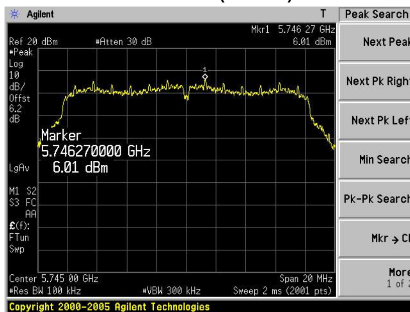
Channel 149 (5745MHz)
