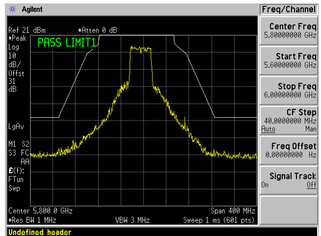
High Channel, 5795 MHz, ANT B
