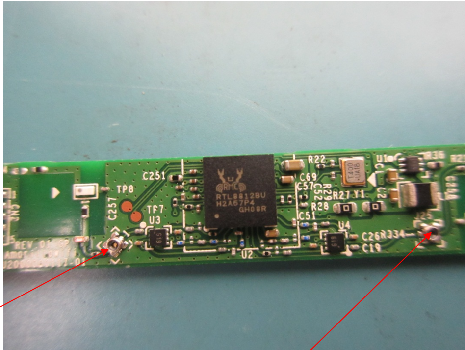
Ant Port 1
