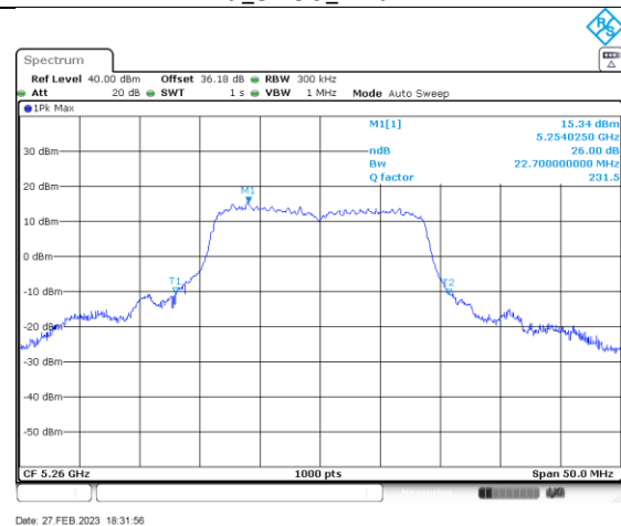
n/ac20_5260_Ant A
