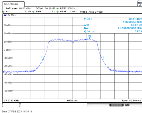
n/ac20_5320_Ant A
