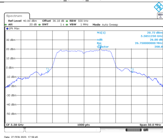
n/ac20_5580_Ant B
