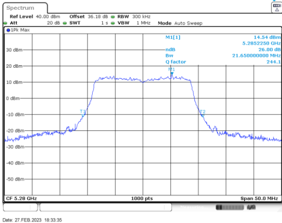
n/ac20_5280_Ant A
