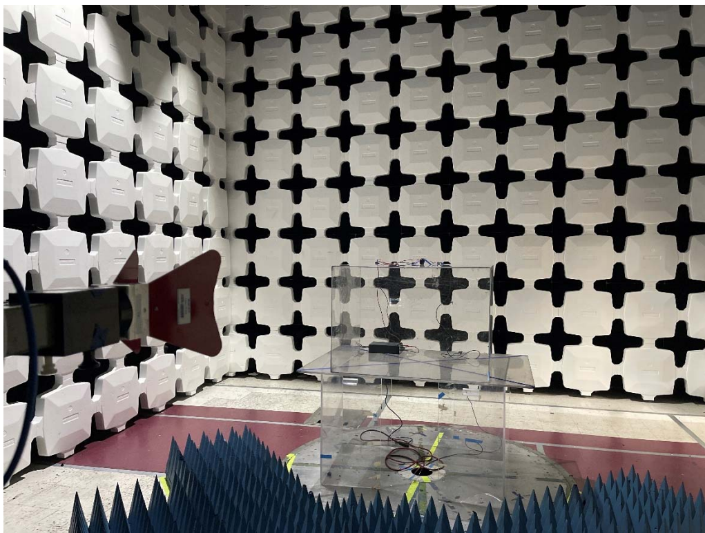
Radiated Emission Test above 1GHz Front View
