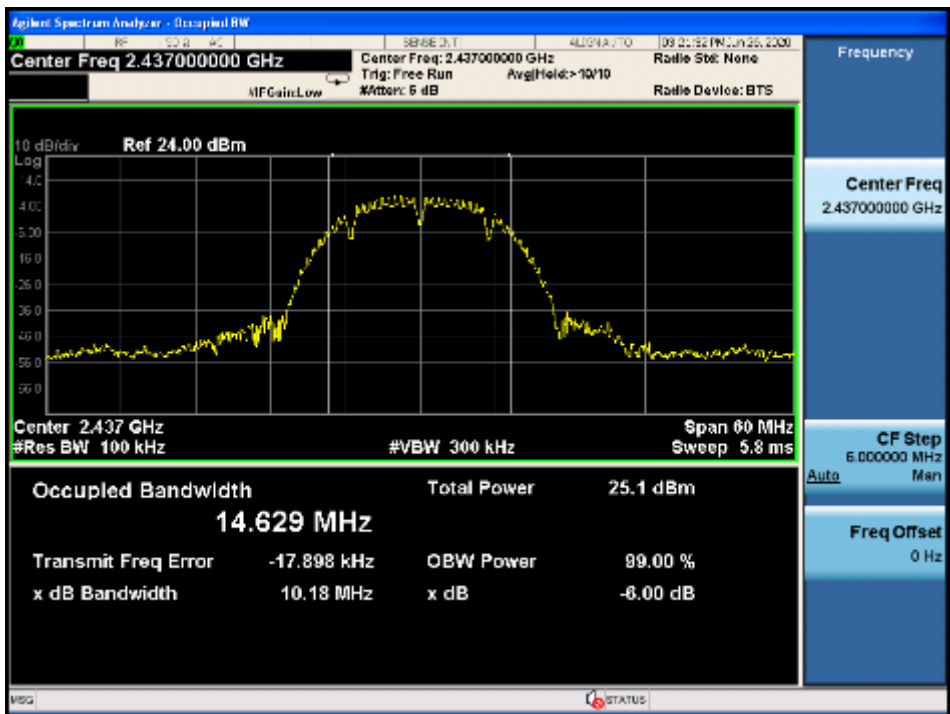
Mid Channel 6 dB OBW Antenna B
