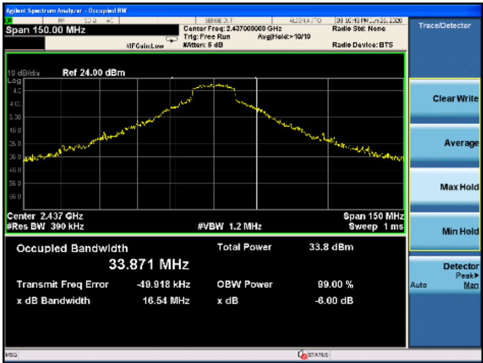
Mid Channel 99% dB OBW Antenna A
