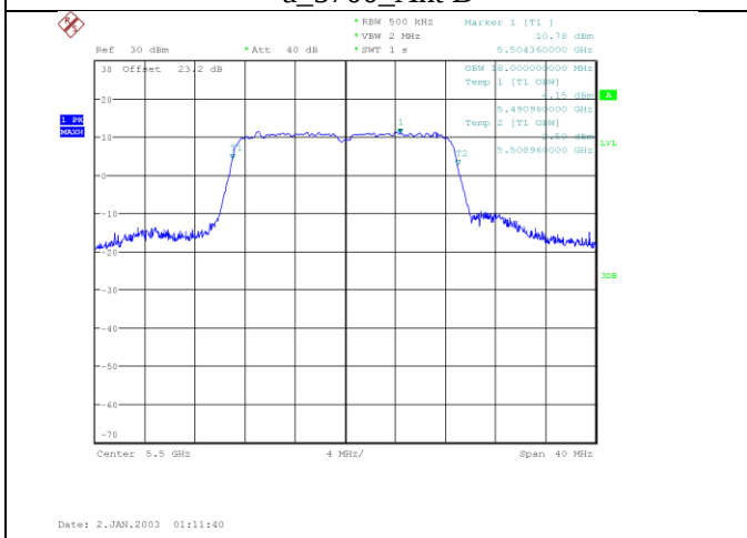
n/ac20_5500_Ant B
