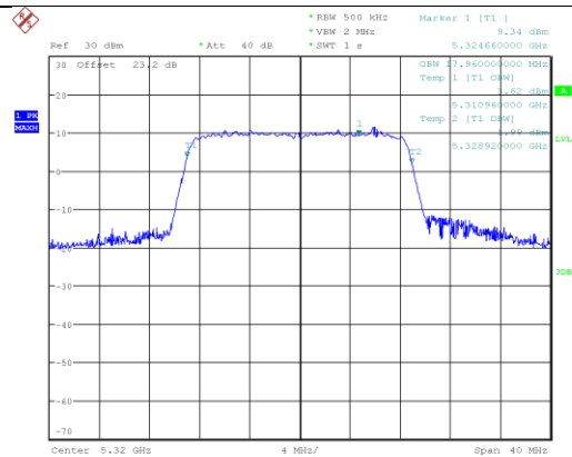
n/ac20_5320_Ant A
