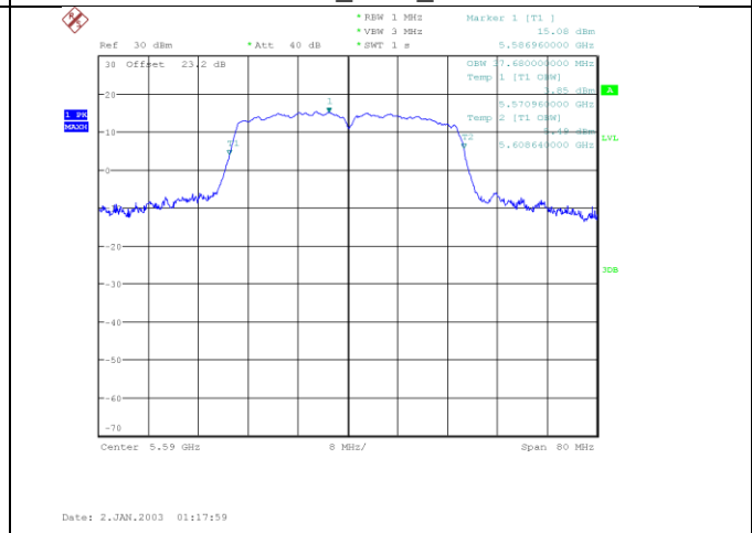
n/ac40_5590_Ant B
