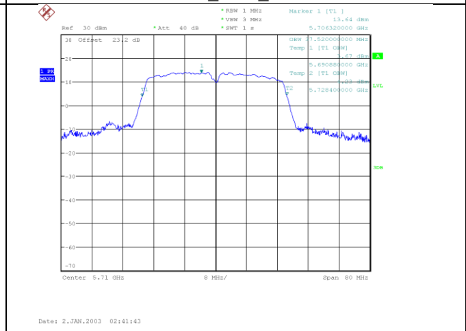
n/ac40_5710_Ant B
