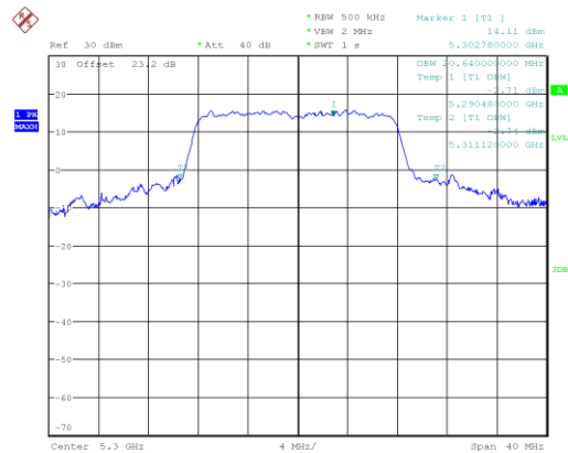
a_5300_Ant B
