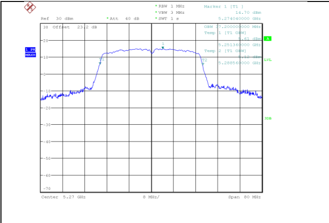
n/ac40_5270_Ant B
