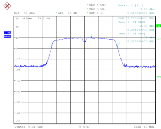
n/ac40_5310_Ant A
