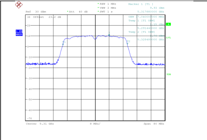
n/ac40_5310_Ant B
