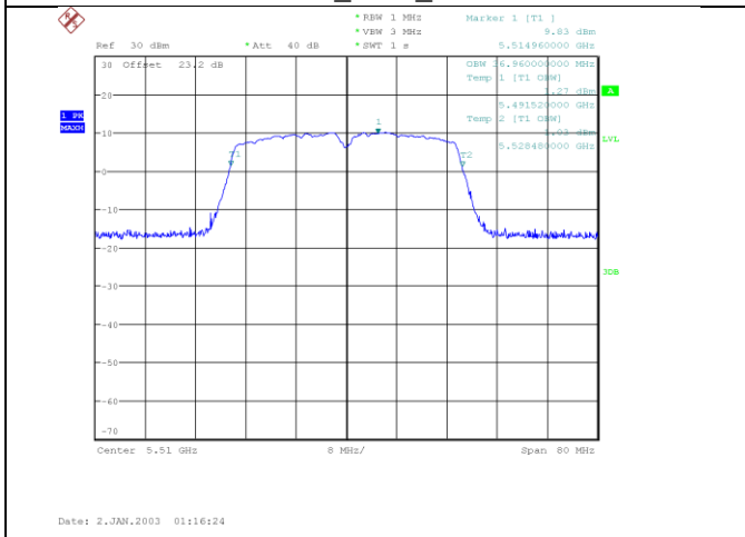
n/ac40_5510_Ant B
