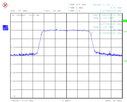
n/ac20_5580_Ant A
