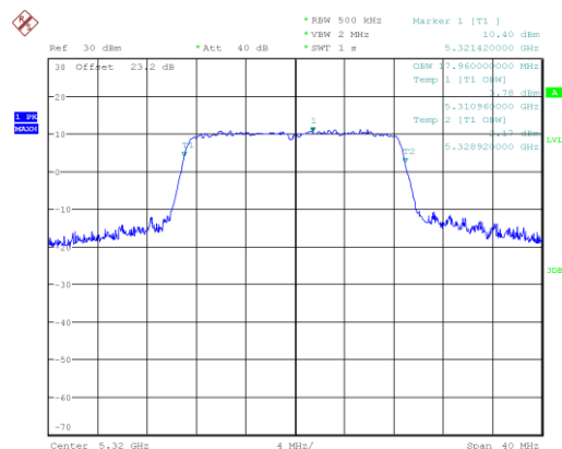
n/ac20_5320_Ant B
