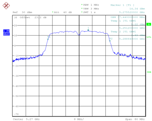
n/ac40_5270_Ant A
