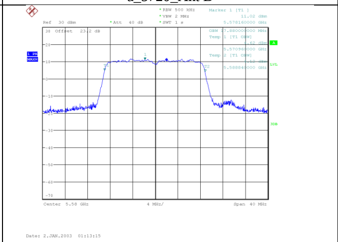
n/ac20_5580_Ant B
