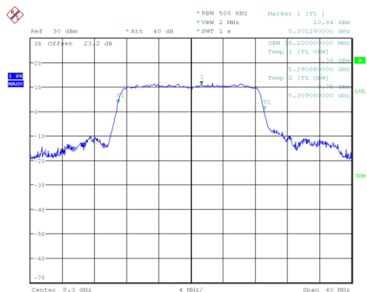
n/ac20_5300_Ant B
