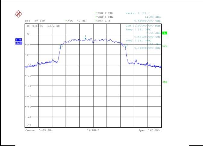
ac80_5690_Ant A
