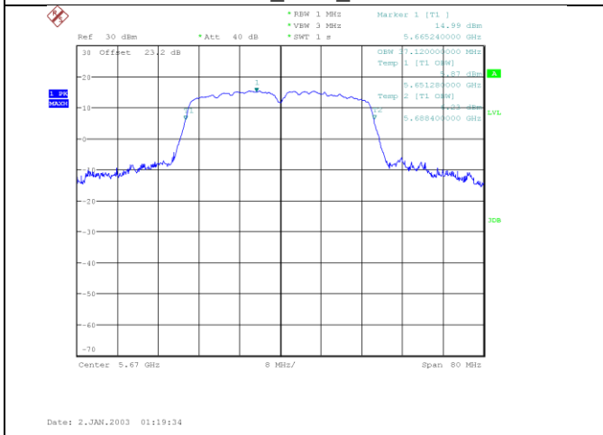
n/ac40_5670_Ant B
