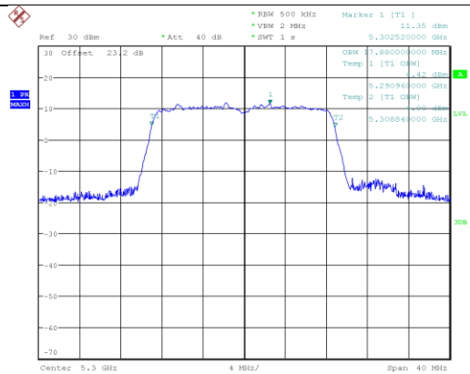
n/ac20_5300_Ant A
