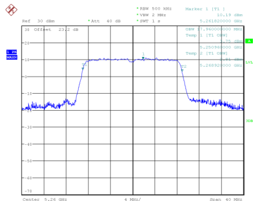
n/ac20_5260_Ant B
