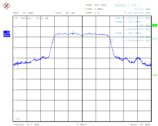
a_5700_Ant A
