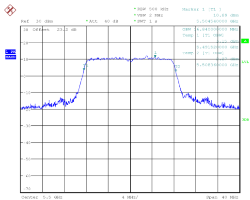
n/ac20_5500_Ant A
