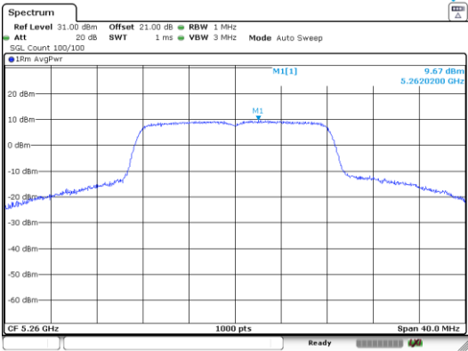
a_5260_Ant A
