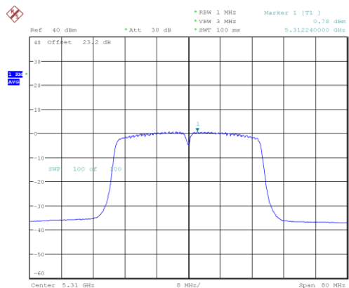
n/ac40_5310_Ant A
