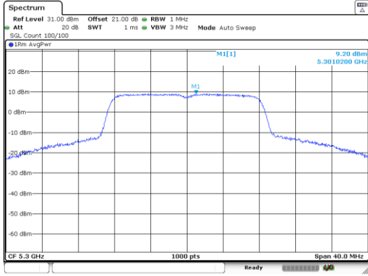
a_5300_Ant A
