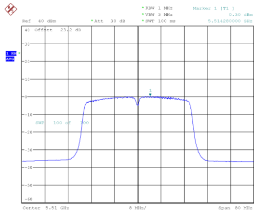
n/ac40_5510_Ant A
