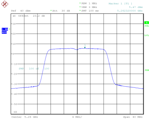
n/ac20_5260_Ant A
