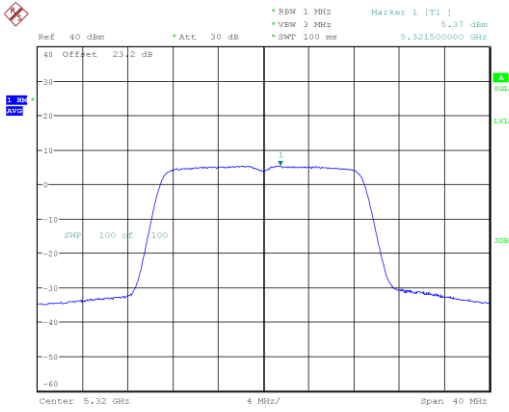
n/ac20_5320_Ant A
