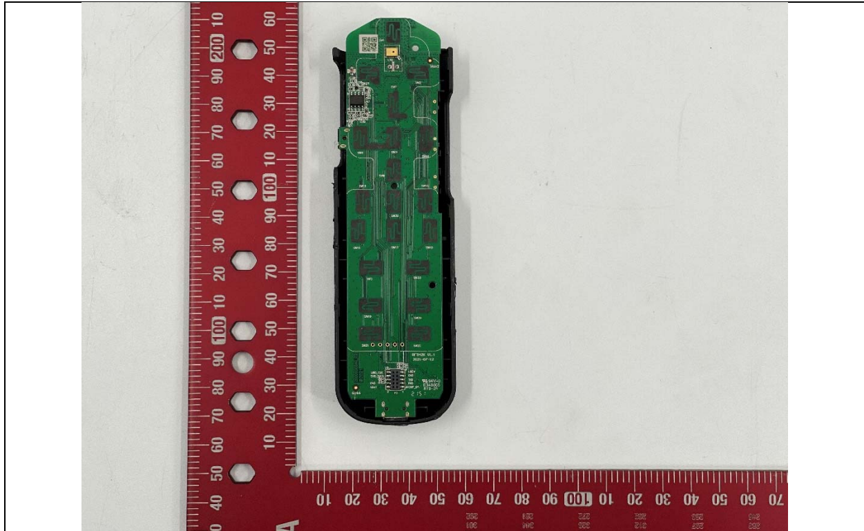
Main Board Top View
