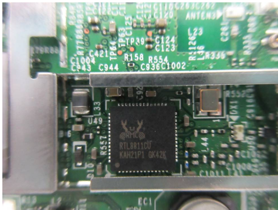
1.5 Internal Top View (Chip Close Up #3)
