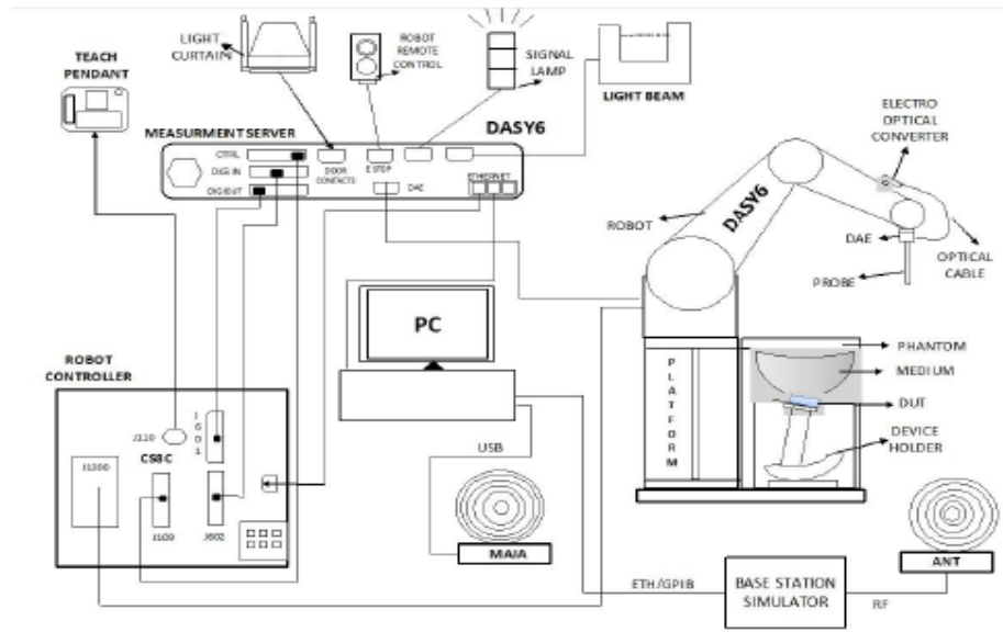
Fig-3.1 SPEAG DASY6 System Setup
