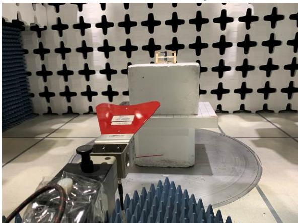
Radiated Emission Test Above 1GHz Front View
