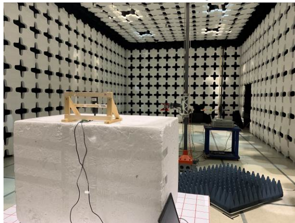
Radiated Emission Test Above 1GHz Rear View
