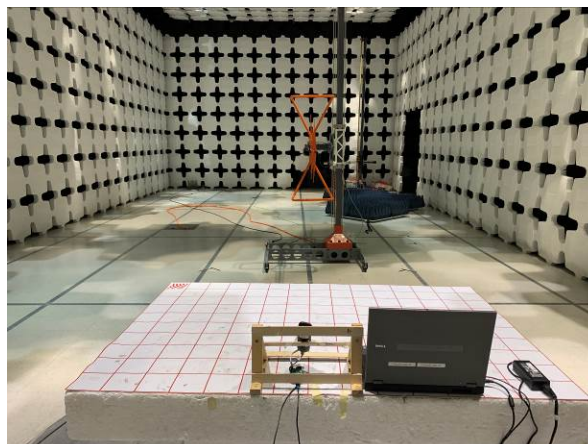
Radiated Emission Test below 1GHz Rear View
