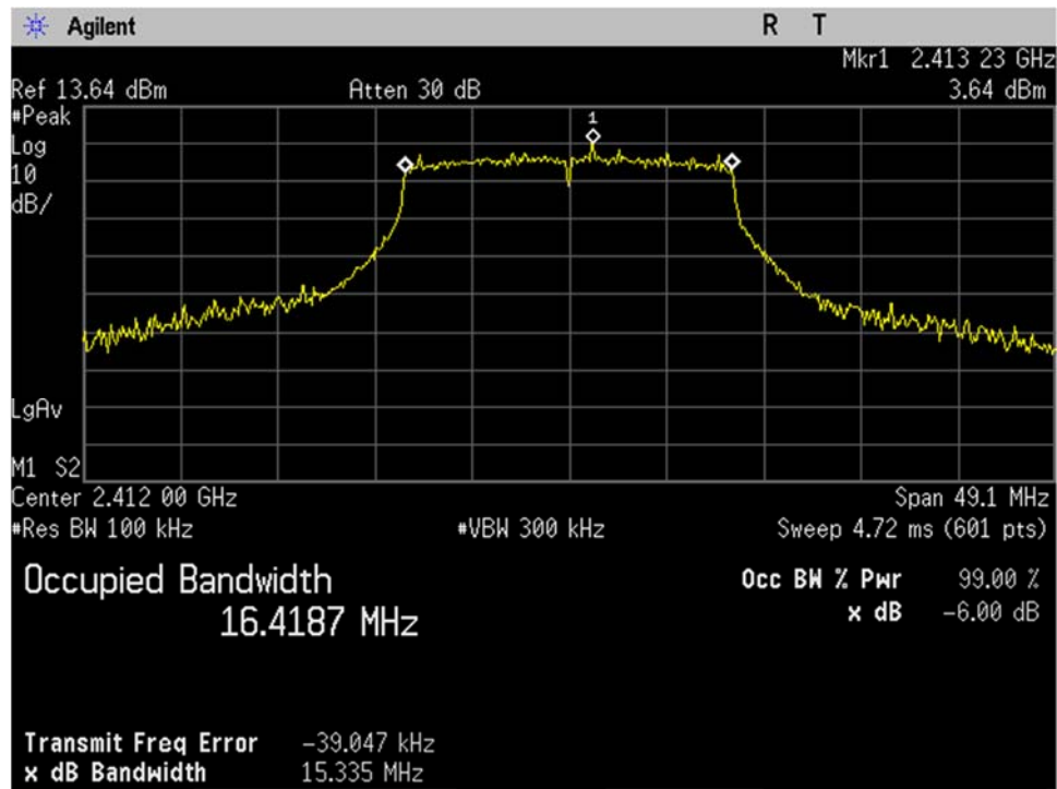
WIFI_Low Ch_2412MHz_20MHz BW_g-mode_Occupied Bandwidth_-6dB_Port 2
