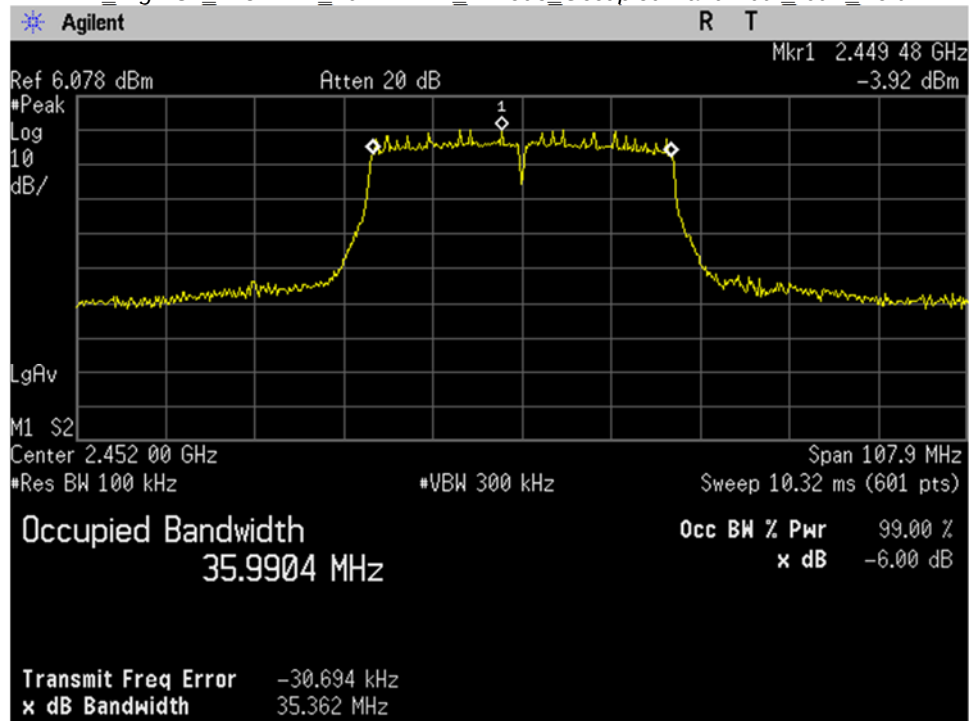
WIFI_High Ch_2452MHz_40MHz BW_n-mode_Occupied Bandwidth_-6dB_Port 2
