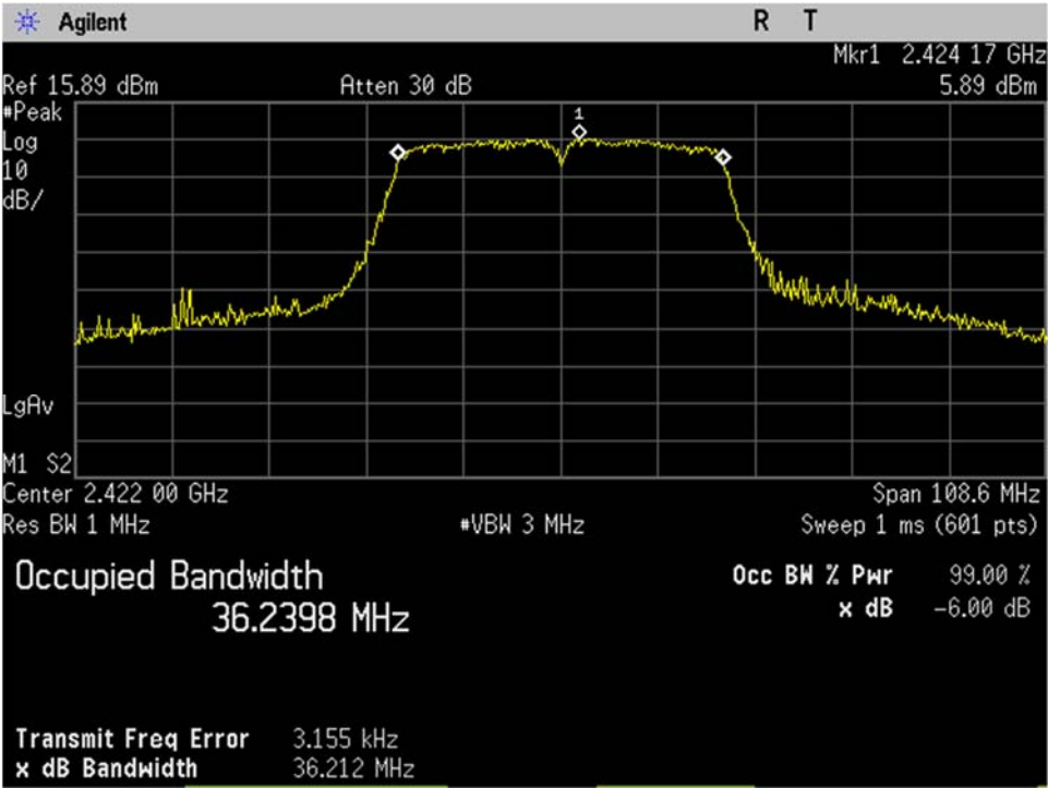
WIFI_Low Ch_2422MHz_40MHz BW_n-mode_Occupied Bandwidth_99 percent_Port 1
