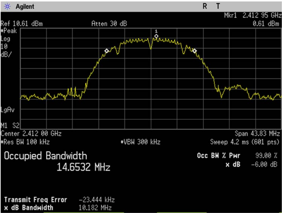
WIFI_Low Ch_2412MHz_20MHz BW_b-mode_Occupied Bandwidth_-6dB_Port 1
