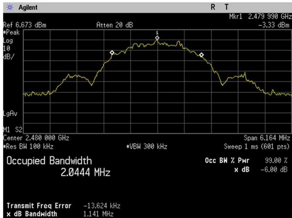
BLE_High Ch_2480MHz_2MBit_Occupied Bandwidth_-6dB_Port 1
