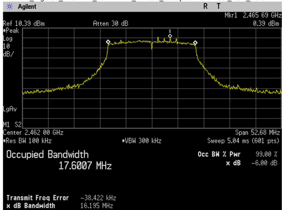
WIFI_High Ch_2462MHz_20MHz BW_n-mode_Occupied Bandwidth_-6dB_Port 2
