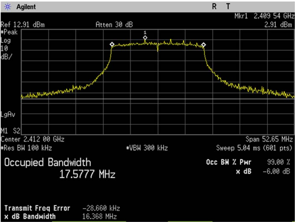
WIFI_Low Ch_2412MHz_20MHz BW_n-mode_Occupied Bandwidth_-6dB_Port 1
