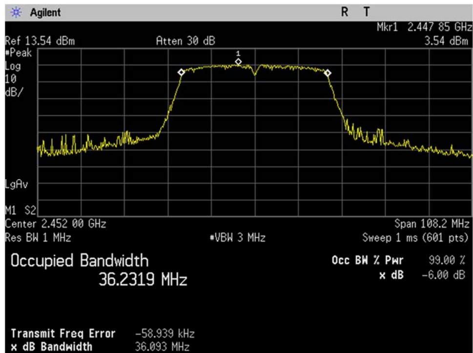
WIFI_High Ch_2452MHz_40MHz BW_n-mode_Occupied Bandwidth_99 percent_Port 2
