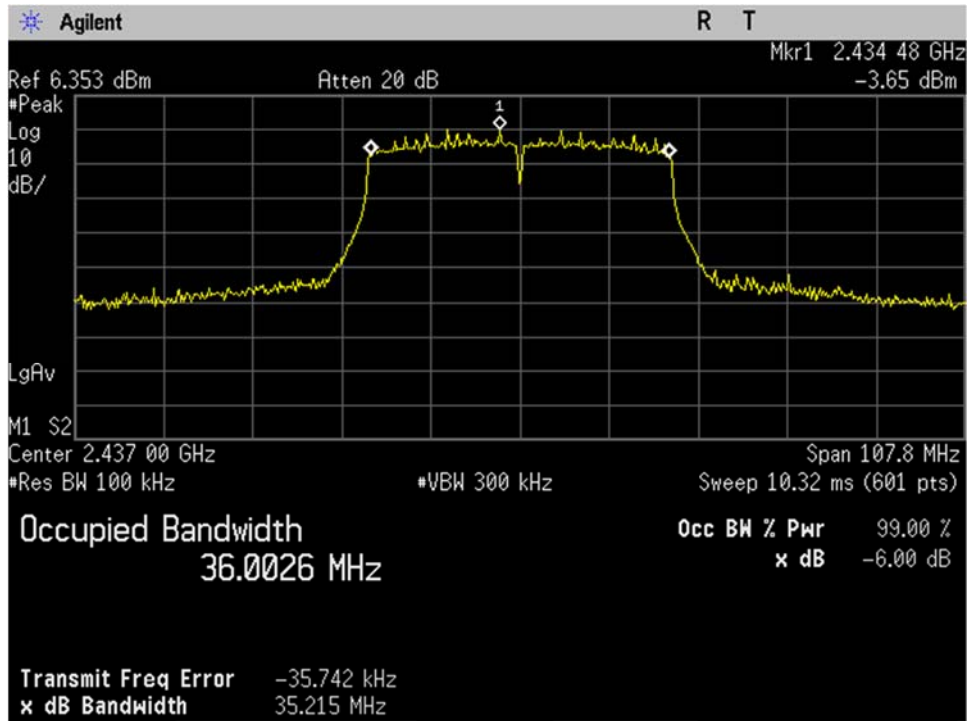
WIFI_Mid Ch_2437MHz_40MHz BW_n-mode_Occupied Bandwidth_-6dB_Port 2
