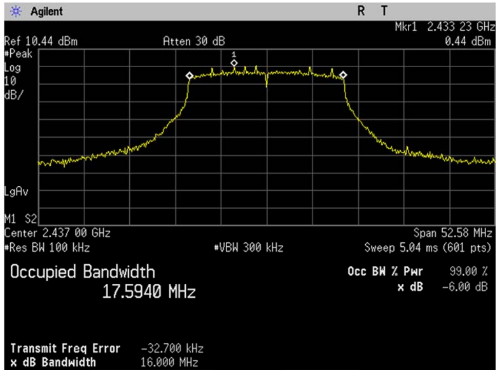
WIFI_Mid Ch_2437MHz_20MHz BW_n-mode_Occupied Bandwidth_-6dB_Port 2
