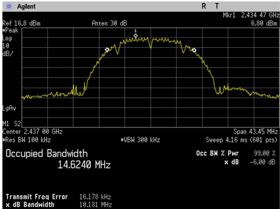
WIFI_Mid Ch_2437MHz_20MHz BW_b-mode_Occupied Bandwidth_-6dB_Port 2
