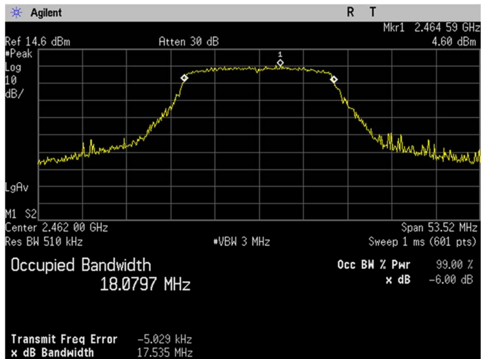
WIFI_High Ch_2462MHz_20MHz BW_n-mode_Occupied Bandwidth_99 percent_Port 2
