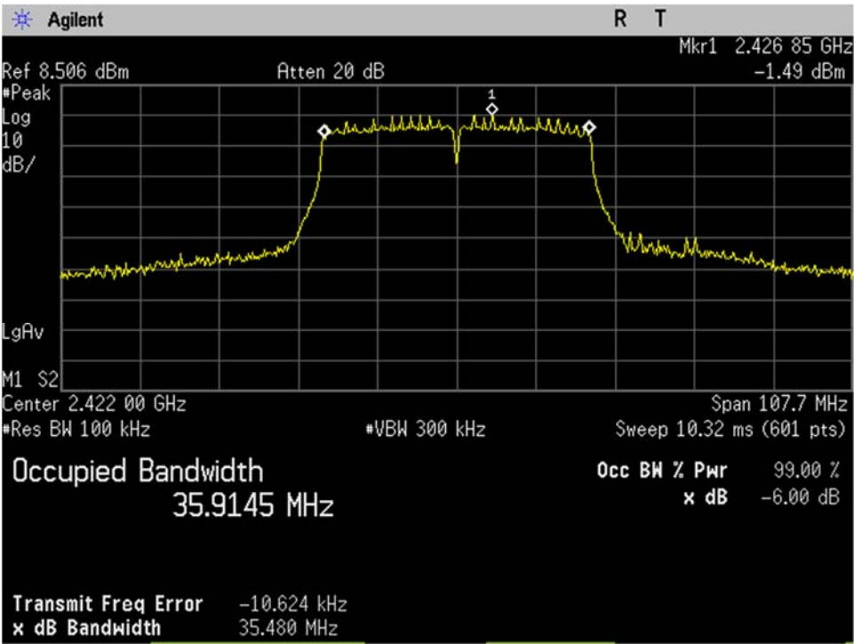
WIFI_Low Ch_2422MHz_40MHz BW_n-mode_Occupied Bandwidth_-6dB_Port 1
