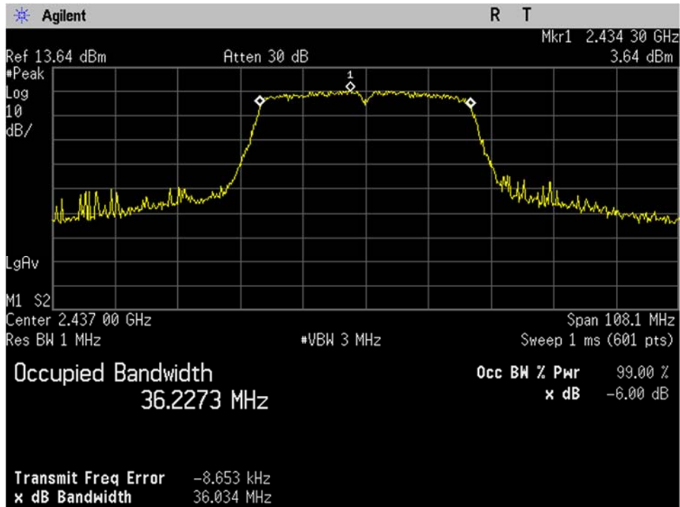
WIFI_Mid Ch_2437MHz_40MHz BW_n-mode_Occupied Bandwidth_99 percent_Port 2
