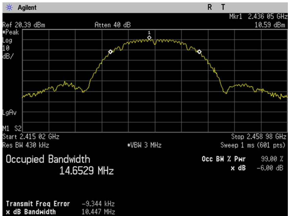
WIFI_Mid Ch_2437MHz_20MHz BW_b-mode_Occupied Bandwidth_99 percent_Port 1
