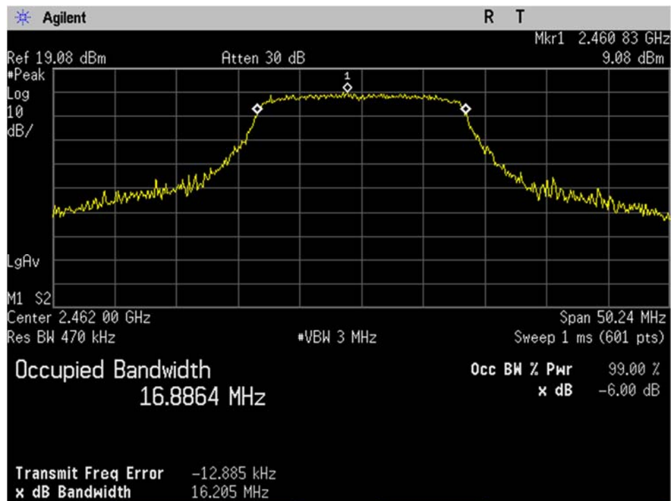
WIFI_High Ch_2462MHz_20MHz BW_g-mode_Occupied Bandwidth_99 percent_Port 1
