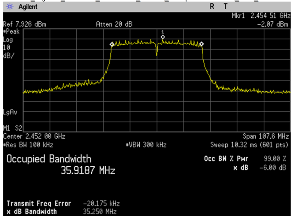
WIFI_High Ch_2452MHz_40MHz BW_n-mode_Occupied Bandwidth_-6dB_Port 1
