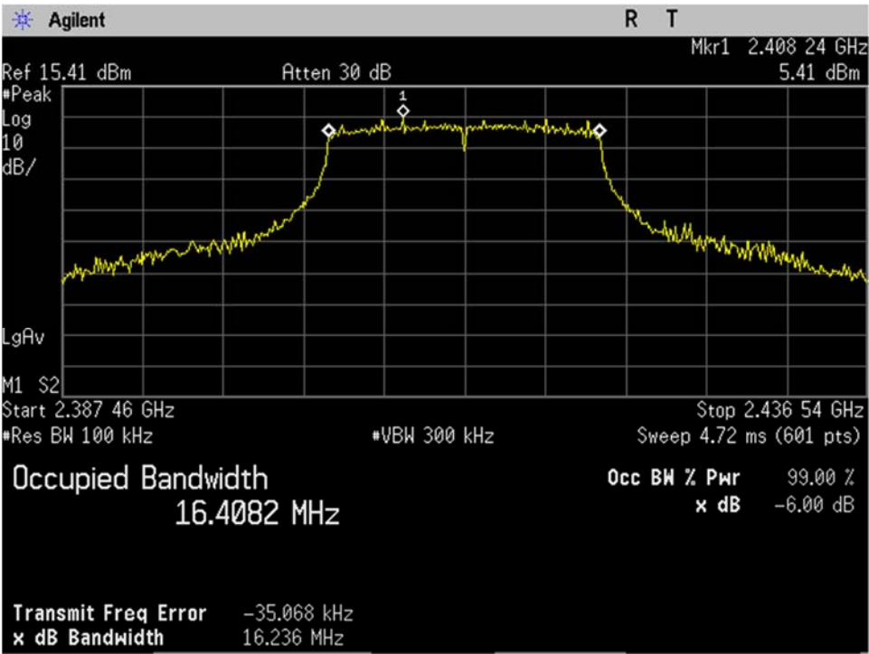
WIFI_Low Ch_2412MHz_20MHz BW_g-mode_Occupied Bandwidth_-6dB_Port 1
