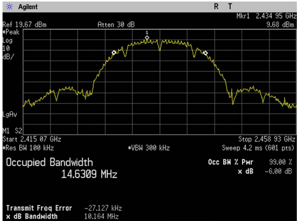
WIFI_Mid Ch_2437MHz_20MHz BW_b-mode_Occupied Bandwidth_-6dB_Port 1
