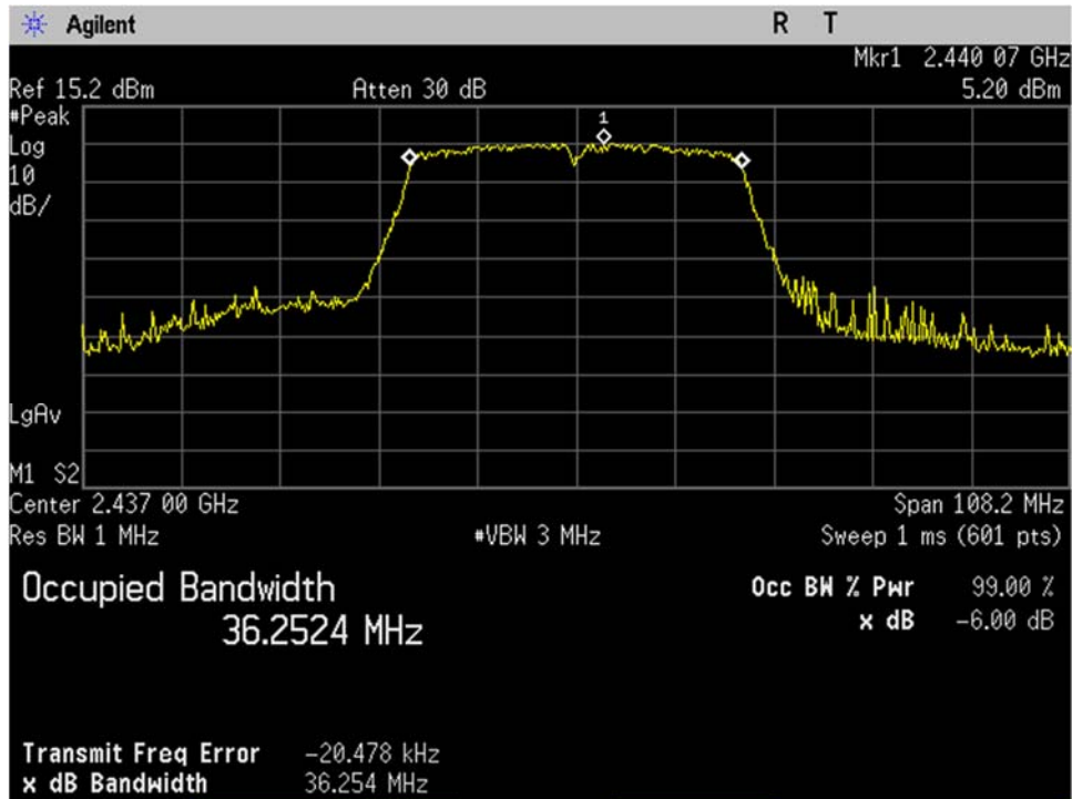
WIFI_Mid Ch_2437MHz_40MHz BW_n-mode_Occupied Bandwidth_99 percent_Port 1
