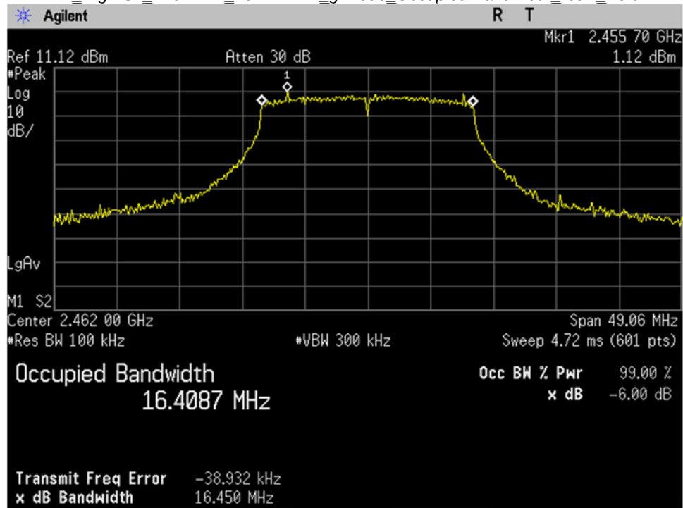
WIFI_High Ch_2462MHz_20MHz BW_g-mode_Occupied Bandwidth_-6dB_Port 2
