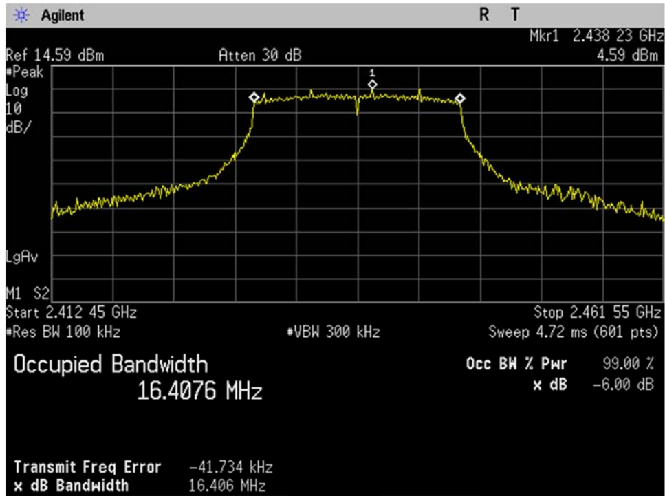
WIFI_Mid Ch_2437MHz_20MHz BW_g-mode_Occupied Bandwidth_-6dB_Port 1
