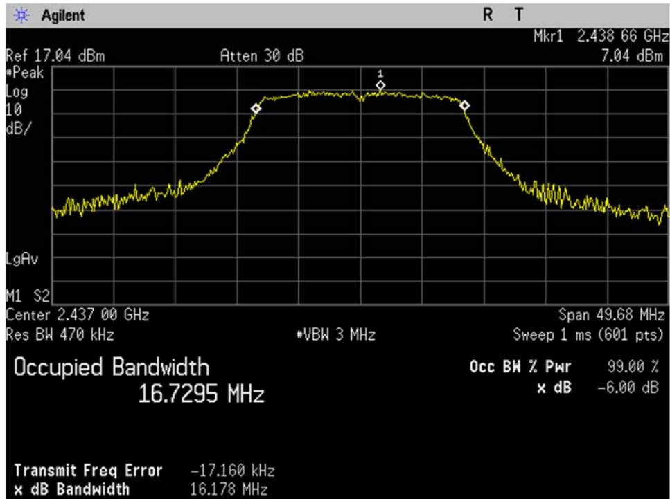
WIFI_Mid Ch_2437MHz_20MHz BW_g-mode_Occupied Bandwidth_99 percent_Port 2
