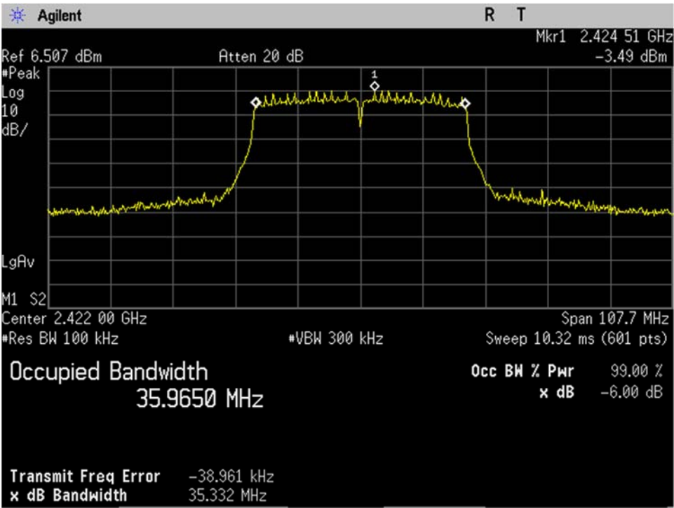
WIFI_Low Ch_2422MHz_40MHz BW_n-mode_Occupied Bandwidth_-6dB_Port 2
