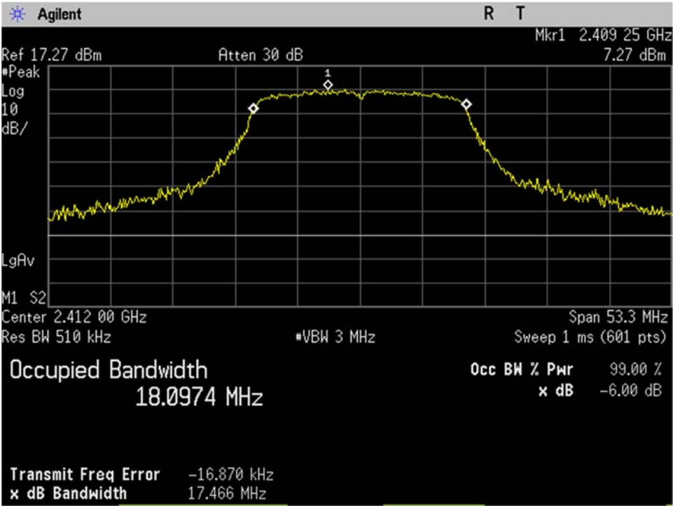
WIFI_Low Ch_2412MHz_20MHz BW_n-mode_Occupied Bandwidth_99 percent_Port 1
