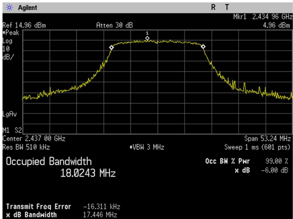
WIFI_Mid Ch_2437MHz_20MHz BW_n-mode_Occupied Bandwidth_99 percent_Port 2
