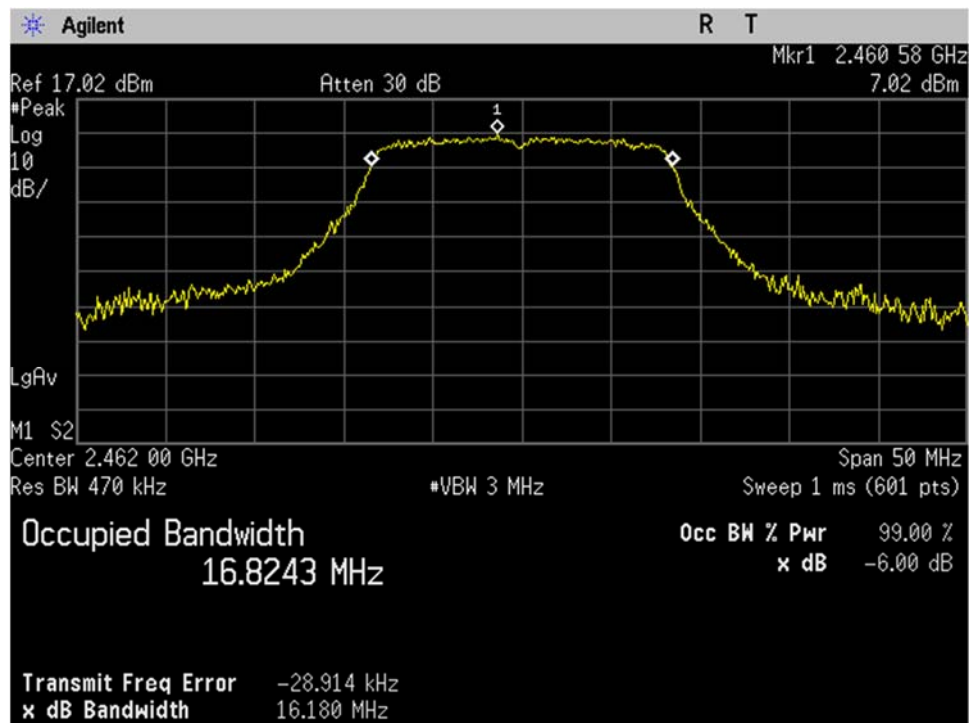
WIFI_High Ch_2462MHz_20MHz BW_g-mode_Occupied Bandwidth_99 percent_Port 2
