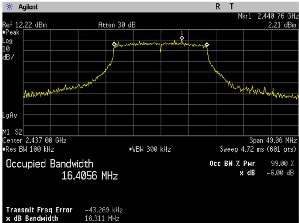
WIFI_Mid Ch_2437MHz_20MHz BW_g-mode_Occupied Bandwidth_-6dB_Port 2
