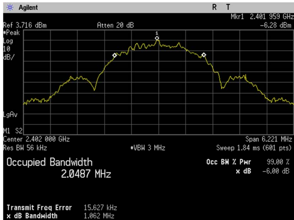
BLE_Low Ch_2402MHz_2MBit_Occupied Bandwidth_99 percent_Port 1
