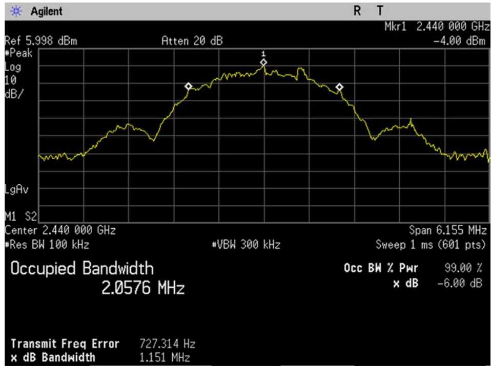
BLE_Mid Ch_2440MHz_2MBit_Occupied Bandwidth_-6dB_Port 1
