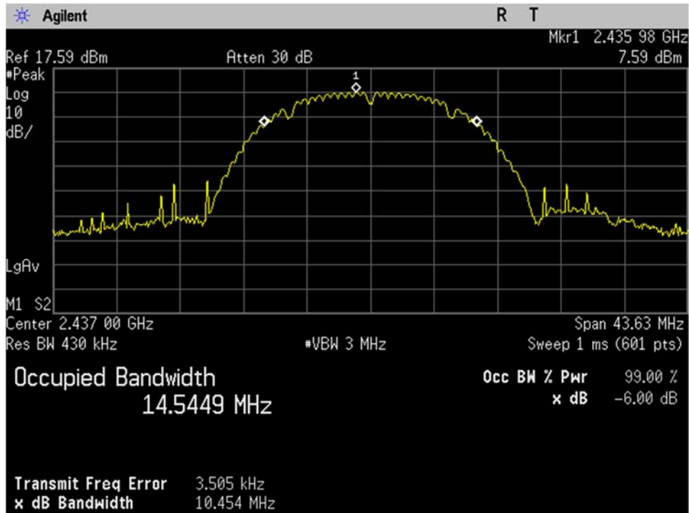
WIFI_Mid Ch_2437MHz_20MHz BW_b-mode_Occupied Bandwidth_99 percent_Port 2
