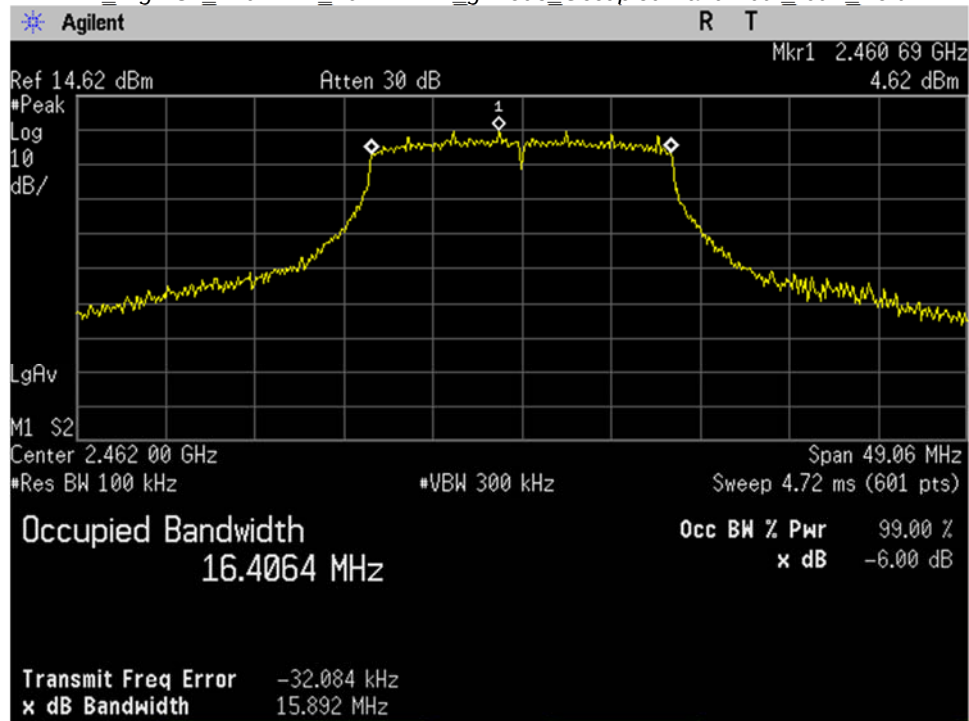
WIFI_High Ch_2462MHz_20MHz BW_g-mode_Occupied Bandwidth_-6dB_Port 1
