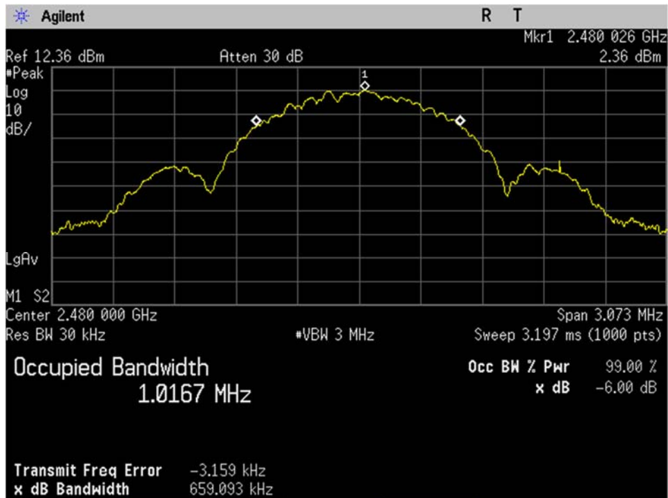
BLE_High Ch_2480MHz_1MBit_Occupied Bandwidth_99 percent_Port 1
