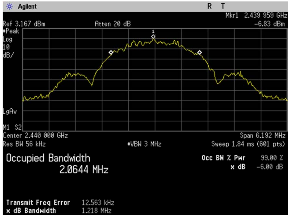
BLE_Mid Ch_2440MHz_2MBit_Occupied Bandwidth_99 percent_Port 1
