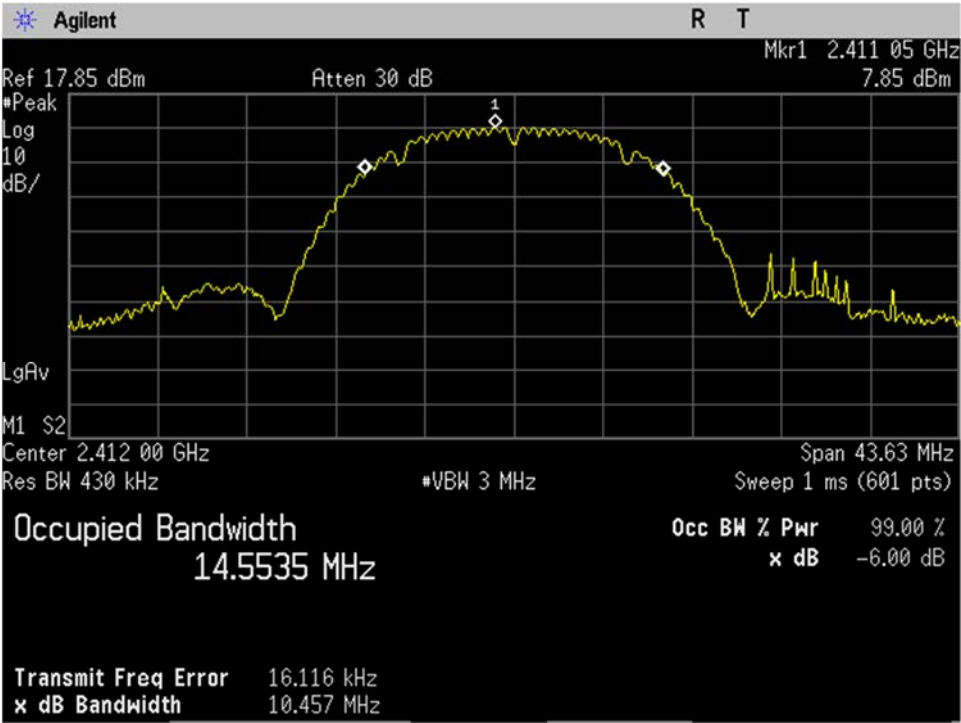
WIFI_Low Ch_2412MHz_20MHz BW_b-mode_Occupied Bandwidth_99 percent_Port 2
