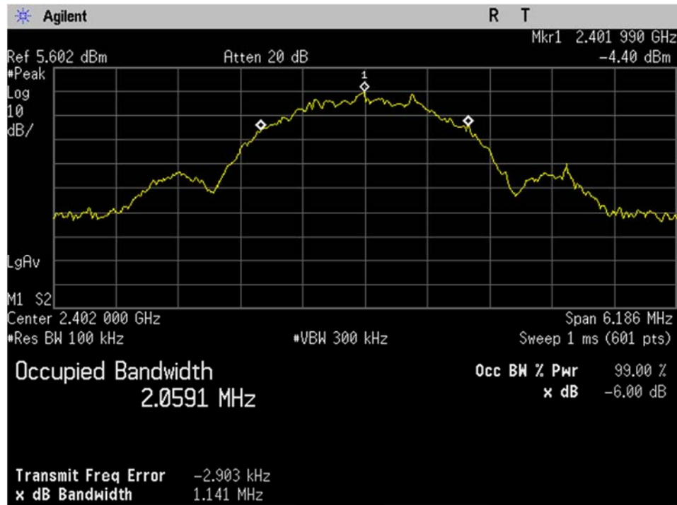
BLE_Low Ch_2402MHz_2MBit_Occupied Bandwidth_-6dB_Port 1
