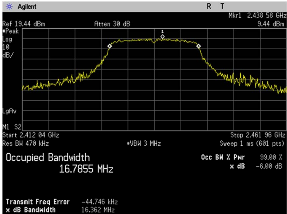
WIFI_Mid Ch_2437MHz_20MHz BW_g-mode_Occupied Bandwidth_99 percent_Port 1
