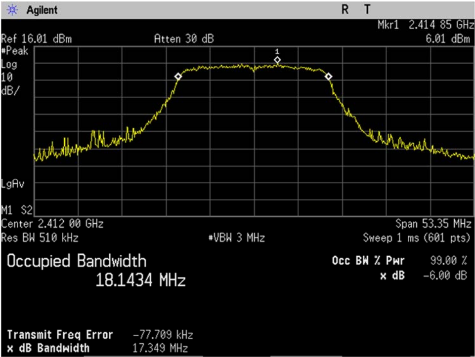
WIFI_Low Ch_2412MHz_20MHz BW_n-mode_Occupied Bandwidth_99 percent_Port 2
