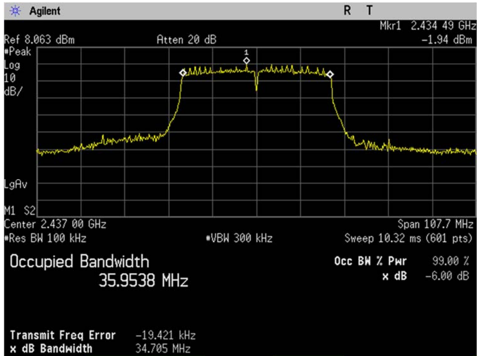
WIFI_Mid Ch_2437MHz_40MHz BW_n-mode_Occupied Bandwidth_-6dB_Port 1
