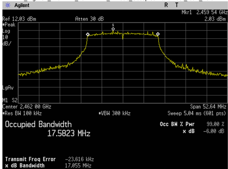
WIFI_High Ch_2462MHz_20MHz BW_n-mode_Occupied Bandwidth_-6dB_Port 1
