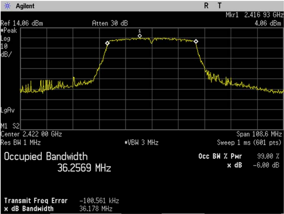
WIFI_Low Ch_2422MHz_40MHz BW_n-mode_Occupied Bandwidth_99 percent_Port 2
