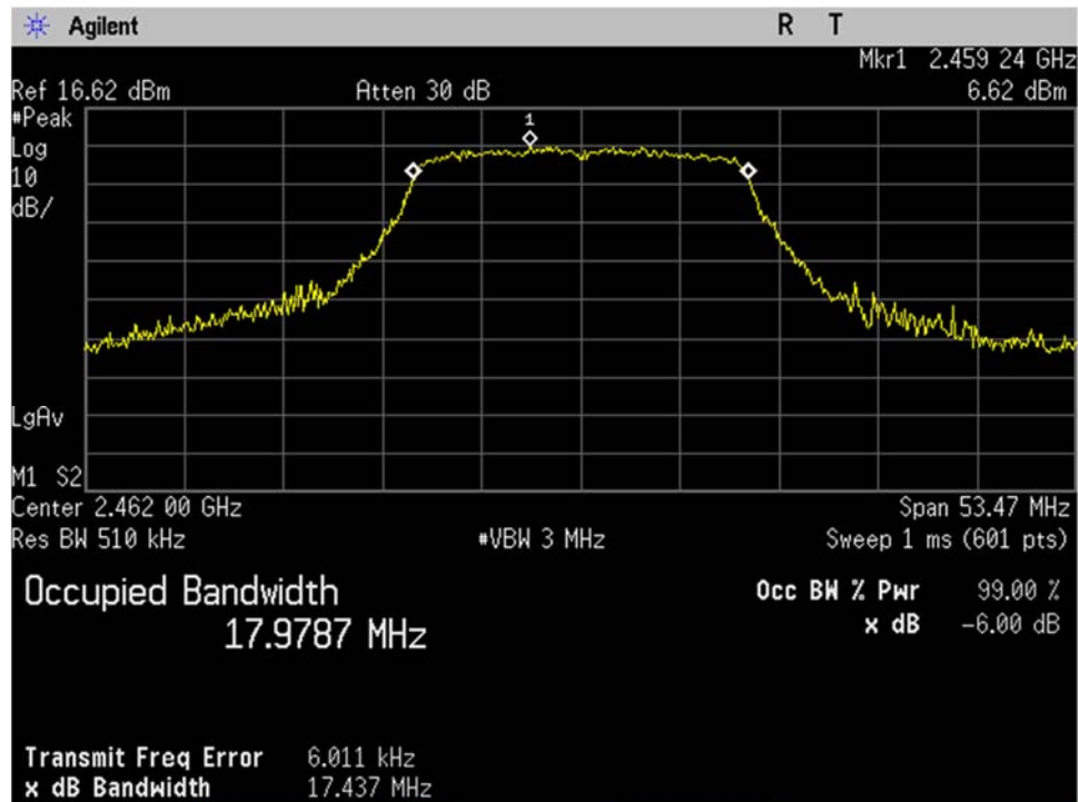
WIFI_High Ch_2462MHz_20MHz BW_n-mode_Occupied Bandwidth_99 percent_Port 1
