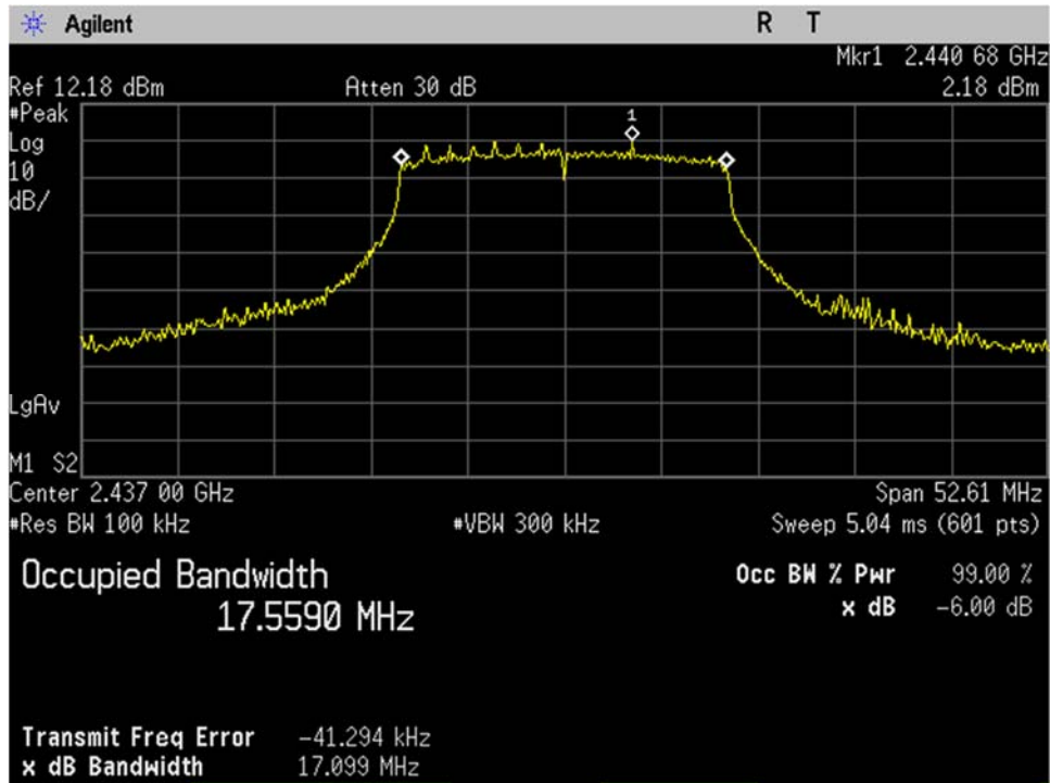
WIFI_Mid Ch_2437MHz_20MHz BW_n-mode_Occupied Bandwidth_-6dB_Port 1
