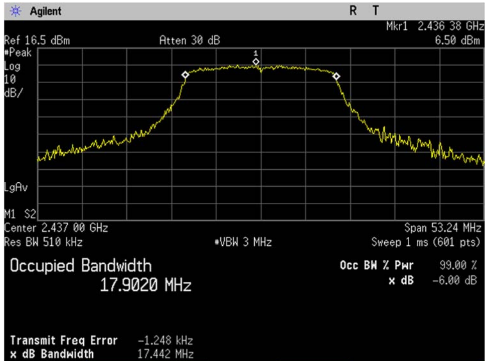
WIFI_Mid Ch_2437MHz_20MHz BW_n-mode_Occupied Bandwidth_99 percent_Port 1
