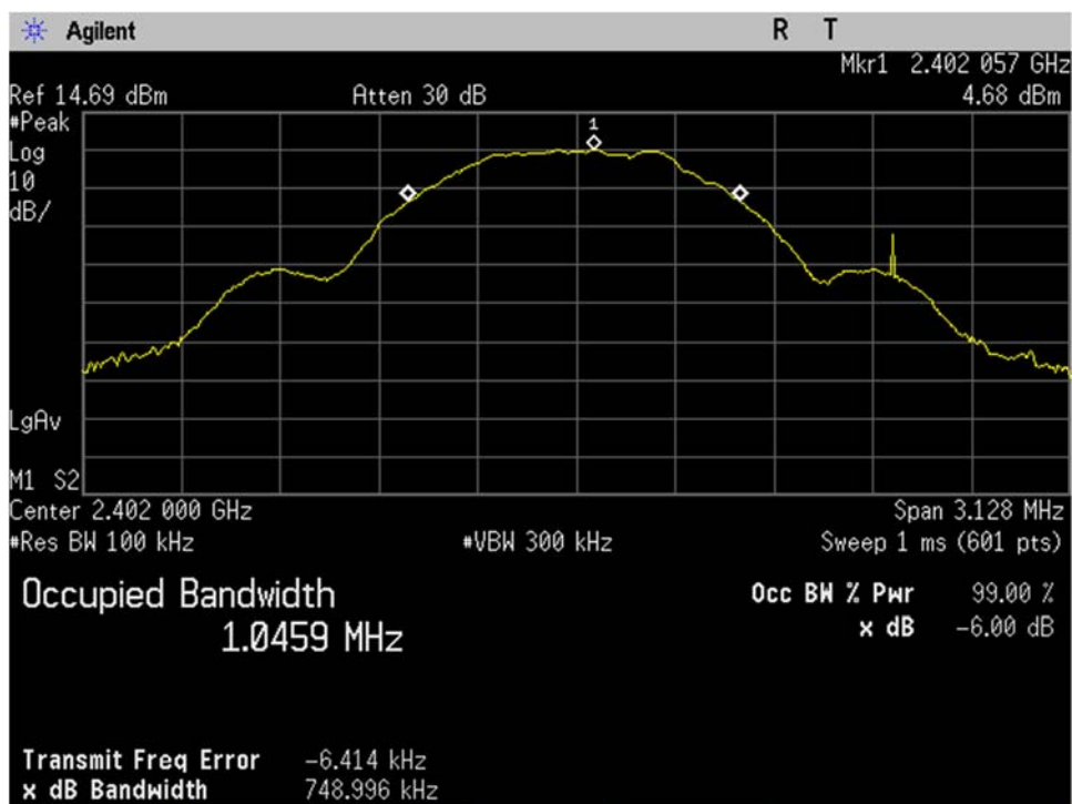
BLE_Low Ch_2402MHz_1MBit_Occupied Bandwidth_99 percent_Port 1
