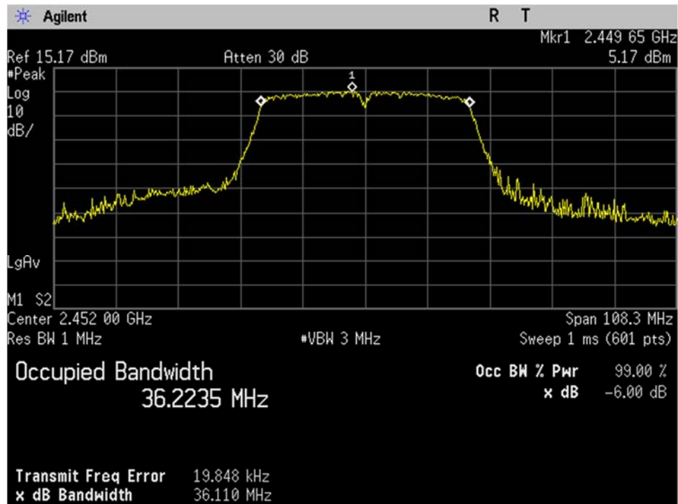
WIFI_High Ch_2452MHz_40MHz BW_n-mode_Occupied Bandwidth_99 percent_Port 1
