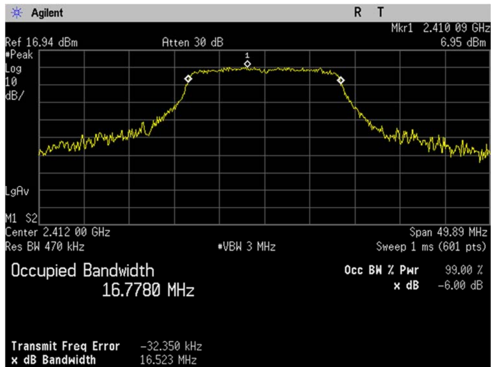
WIFI_Low Ch_2412MHz_20MHz BW_g-mode_Occupied Bandwidth_99 percent_Port 2
