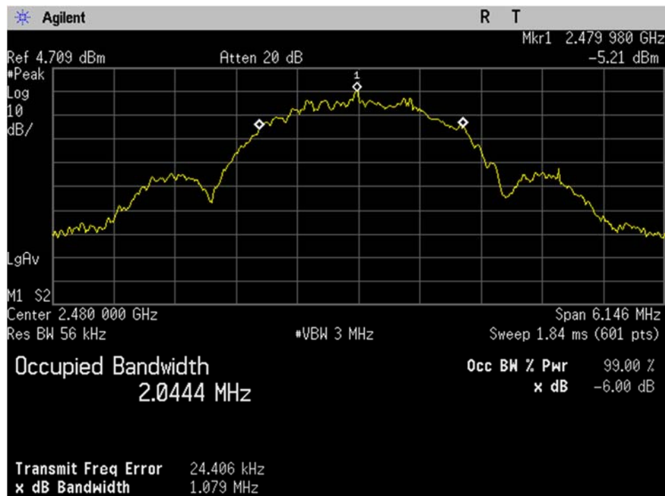
BLE_High Ch_2480MHz_2MBit_Occupied Bandwidth_99 percent_Port 1
