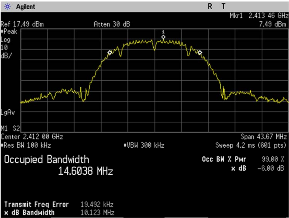
WIFI_Low Ch_2412MHz_20MHz BW_b-mode_Occupied Bandwidth_-6dB_Port 2
