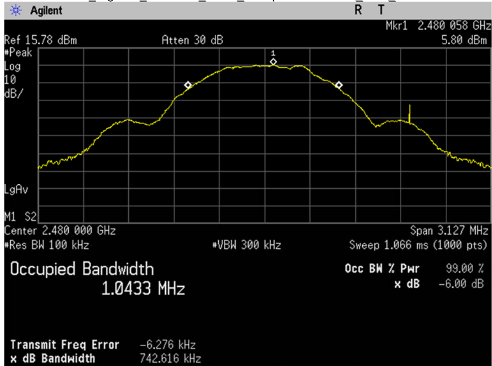
BLE_High Ch_2480MHz_1MBit_Occupied Bandwidth_-6dB_Port 1
