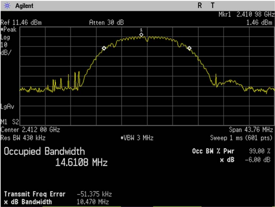
WIFI_Low Ch_2412MHz_20MHz BW_b-mode_Occupied Bandwidth_99 percent_Port 1
