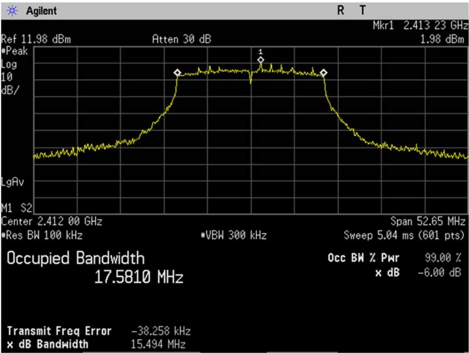
WIFI_Low Ch_2412MHz_20MHz BW_n-mode_Occupied Bandwidth_-6dB_Port 2
