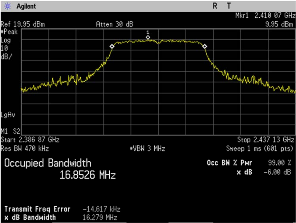
WIFI_Low Ch_2412MHz_20MHz BW_g-mode_Occupied Bandwidth_99 percent_Port 1
