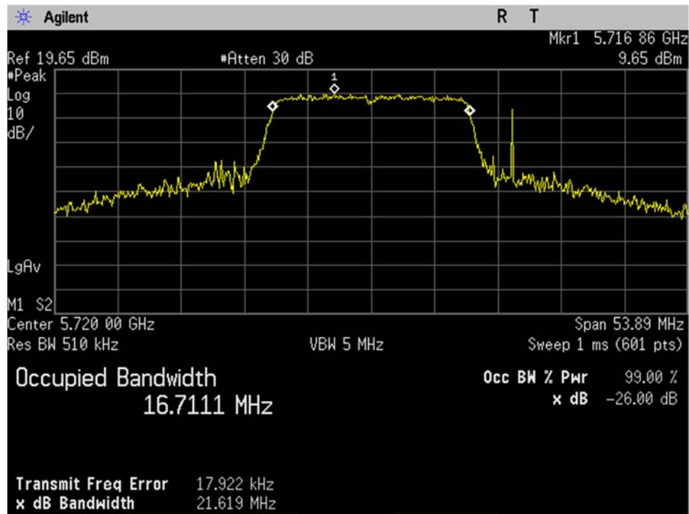
U-NII-2C_5720MHz_High Ch_144_20MHz BW_a-mode_Occupied Bandwidth_-26dB_Port 1
