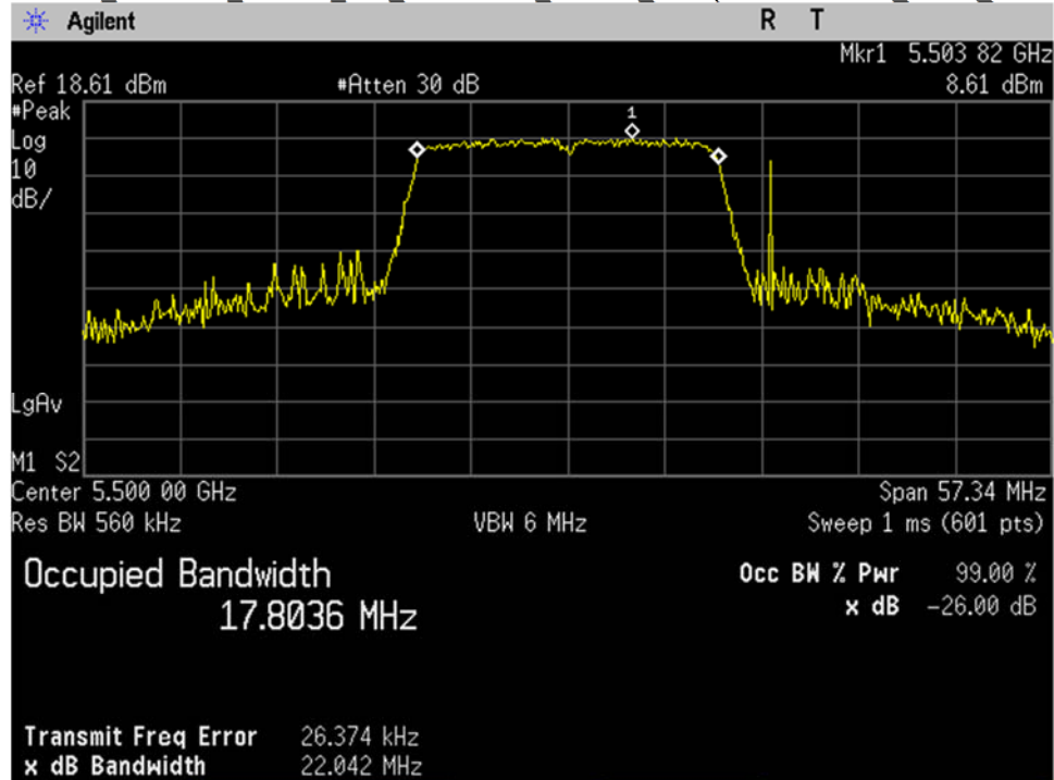
U-NII-2C_5500MHz_Low Ch_100_20MHz BW_n-mode_Occupied Bandwidth_-26dB_Port 2
