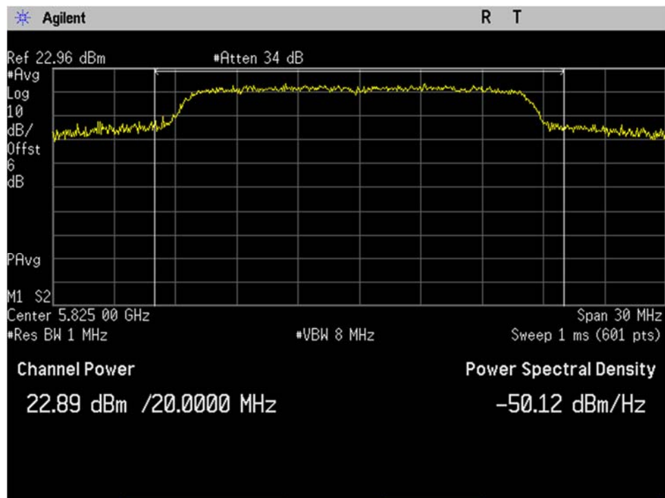
U-NII-3_5825MHz_High Ch_165_20MHz BW_a-mode_Output Power_Port 2
