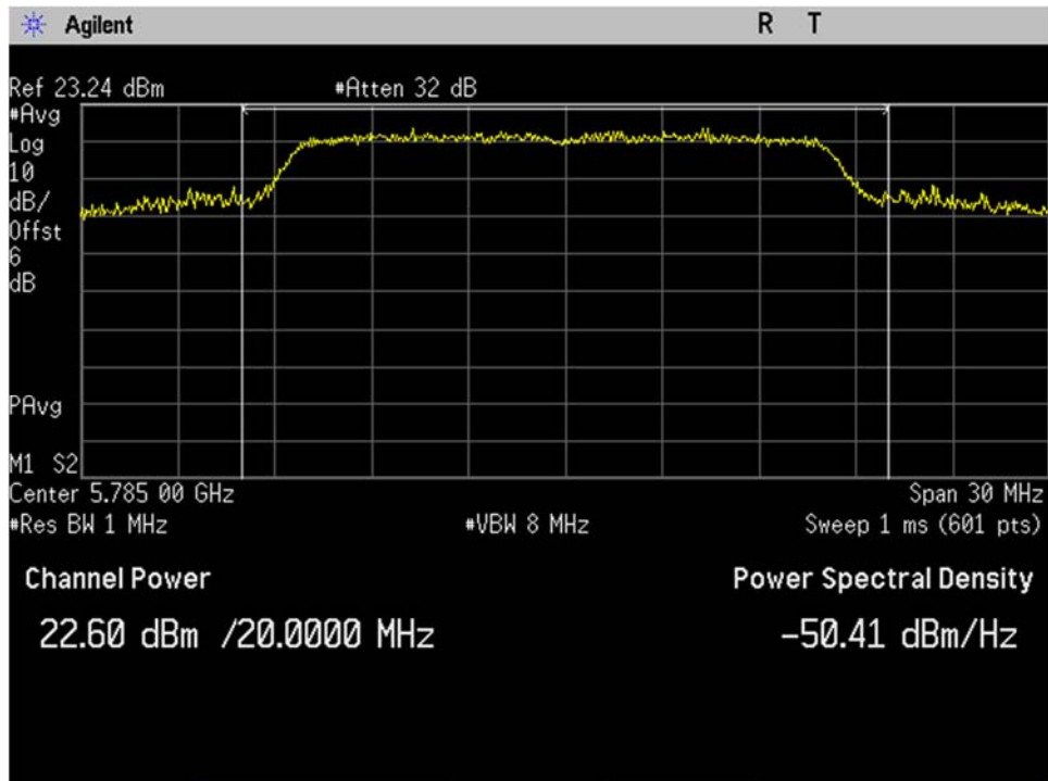
U-NII-3_5785MHz_Mid Ch_157_20MHz BW_a-mode_Output Power_Port 2
