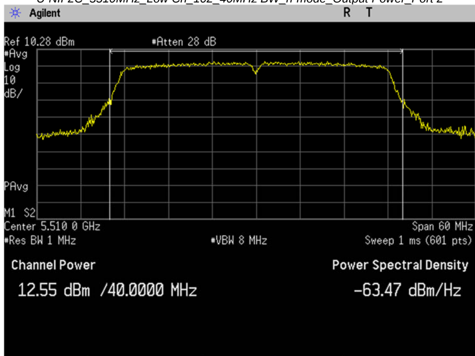
U-NII-2C_5510MHz_Low Ch_102_40MHz BW_n-mode_Output Power_Port 2
