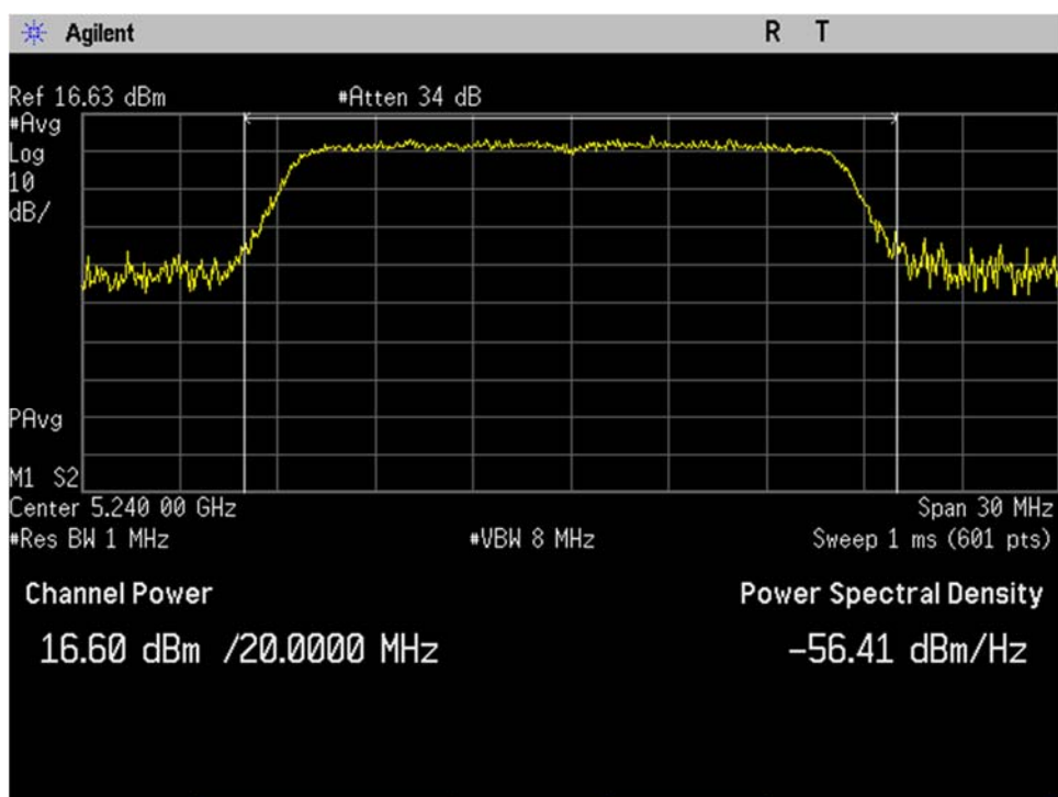
U-NII-1_5240MHz_high_mid Ch_48_20MHz BW_a-mode_Output Power_Port 2
