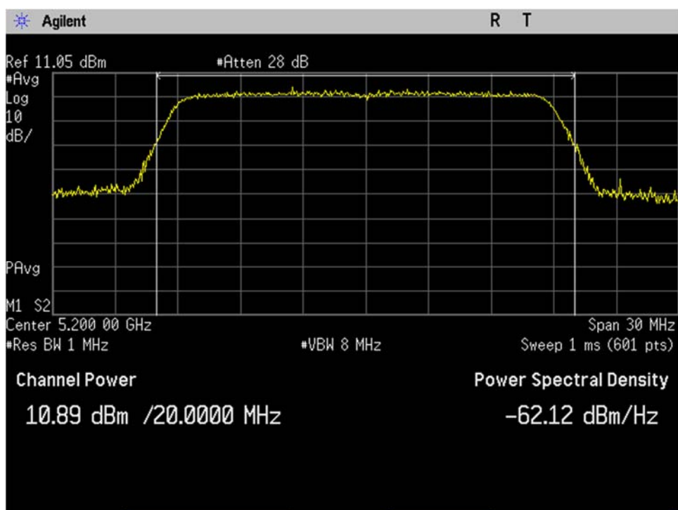
U-NII-1_5200MHz_low_Mid Ch_40_20MHz BW_n-mode_Output Power_Port 2
