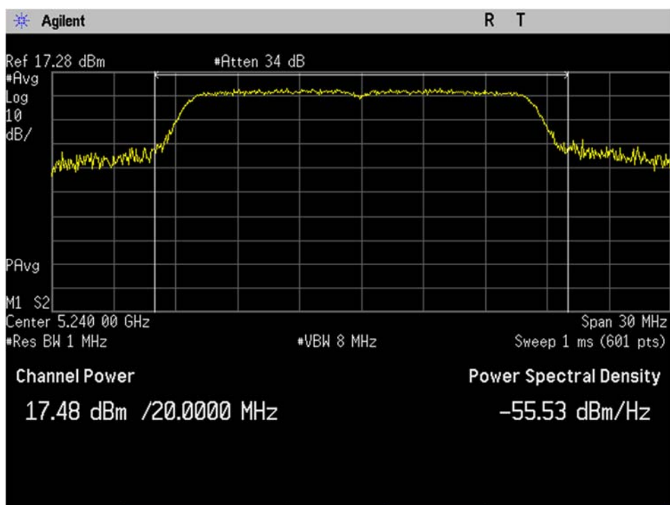
U-NII-1_5240MHz_high_mid Ch_48_20MHz BW_a-mode_Output Power_Port 1
