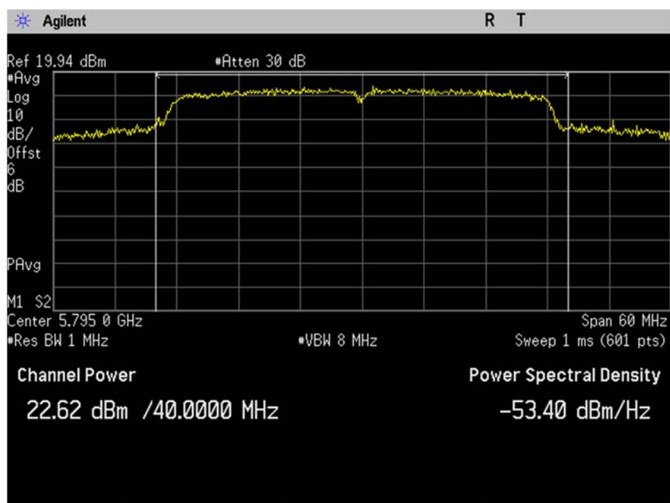
U-NII-3_5795MHz_High_Mid_Ch_159_40MHz BW_n-mode_Output Power_Port 1
