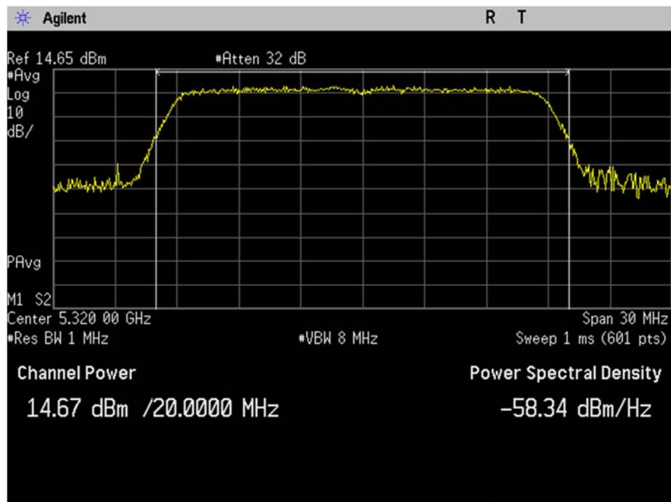
U-NII-2A_5320MHz_High Ch_64_20MHz BW_n-mode_Output Power_Port 2
