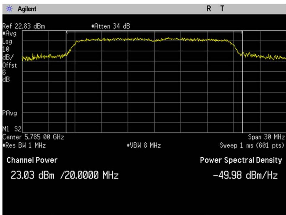
U-NII-3_5785MHz_Mid Ch_157_20MHz BW_n-mode_Output Power_Port 2
