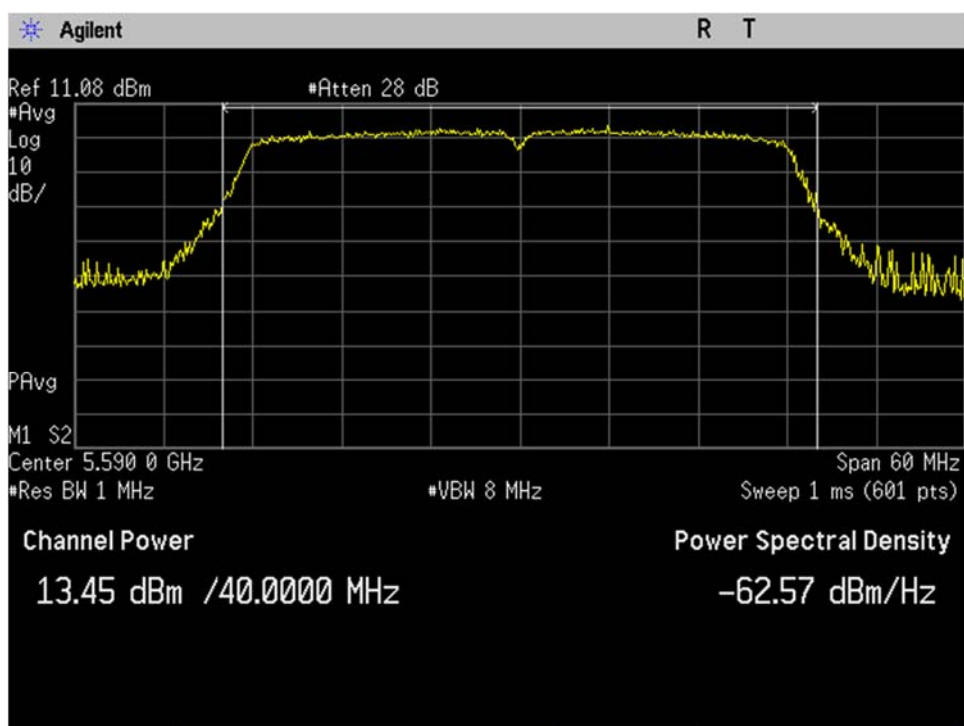
U-NII-2C_5590MHz_Mid Ch_118_40MHz BW_n-mode_Output Power_Port 2
