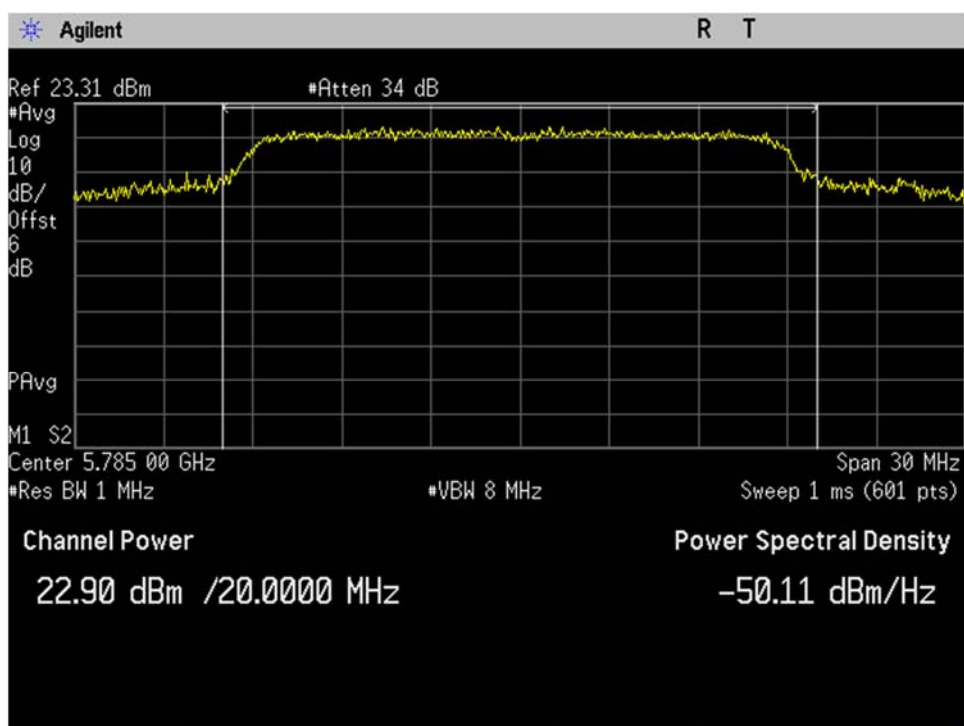
U-NII-3_5785MHz_Mid Ch_157_20MHz BW_n-mode_Output Power_Port 1
