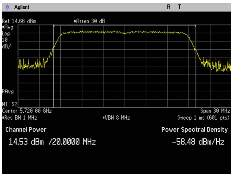
U-NII-2C_5720MHz_High Ch_144_20MHz BW_n-mode_Output Power_Port 2
