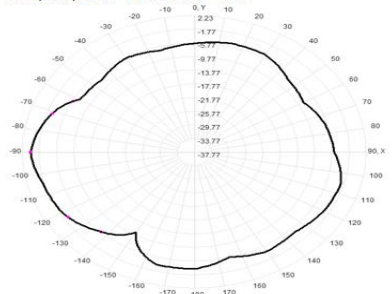
Total(H-XY), Max= 0.26dBi, CirD=10.96
