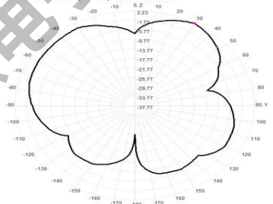
5850.0MHz Total(E2-YZ), Max= 2.23dBi
