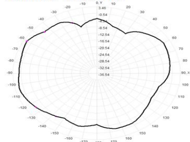
Total(H-XY), Max= 1.89dBi, CirD=11.03
