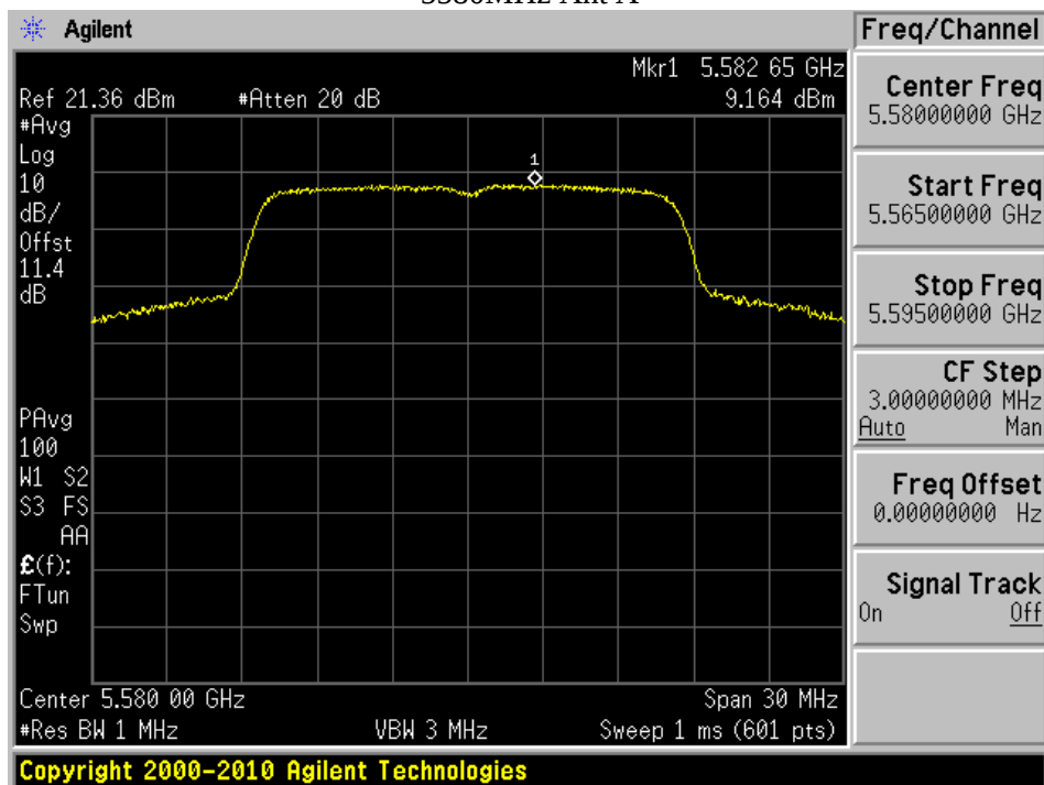
5580MHz Ant A
