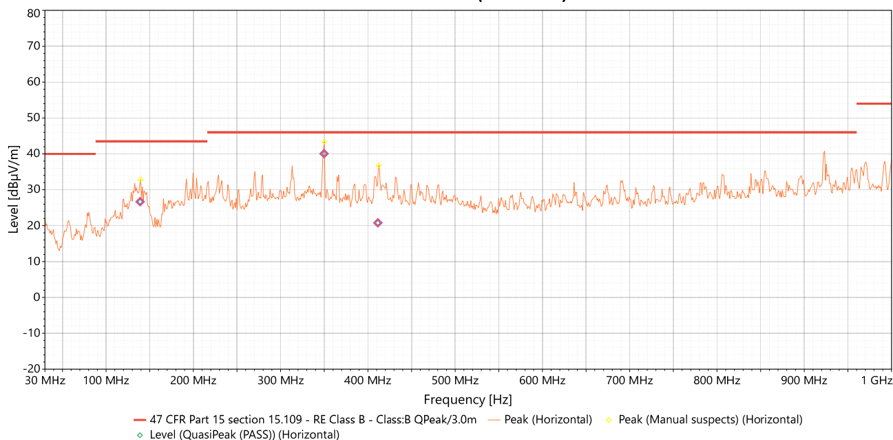
#2 - 30MHz-1GHz (Horizontal)
