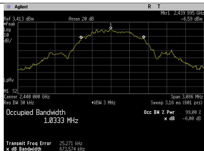
BLE_Mid Ch_2440MHz_1MBit_Occupied Bandwidth_99 percent_Port 1
