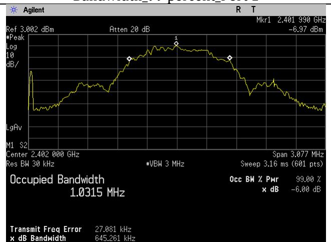
BLE_Low Ch_2402MHz_1MBit_Occupied Bandwidth_99 percent_Port 1
