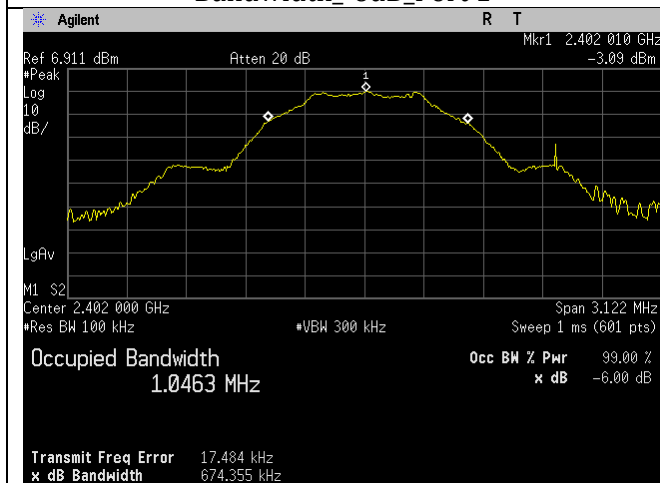
BLE_Low Ch_2402MHz_1MBit_Occupied Bandwidth_-6dB_Port 1
