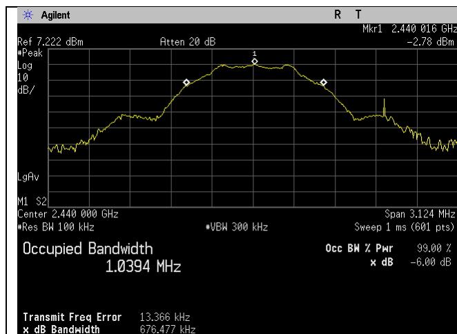
BLE_Mid Ch_2440MHz_1MBit_Occupied Bandwidth_-6dB_Port 1
