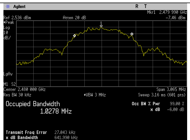
BLE_High Ch_2480MHz_1MBit_Occupied Bandwidth_99 percent_Port 1
