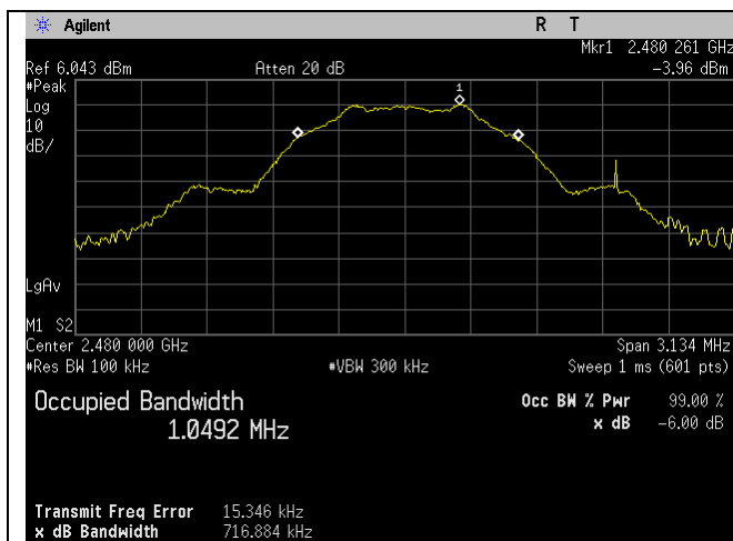
BLE_High Ch_2480MHz_1MBit_Occupied Bandwidth_-6dB_Port 1
